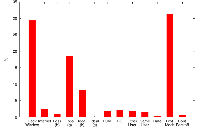
Figure 5: Root wireless causes that limit TCP flow throughput.
