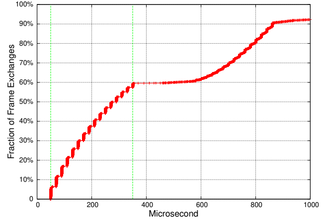
Figure 3: Access delay ( d_{acc} ) distribution of one hour of frame exchanges from an AP to a client doing a bulk TCP download.
