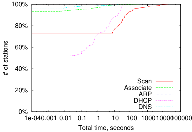
Figure 12: CDF of delays experienced by 802.11 clients due to timeouts.
