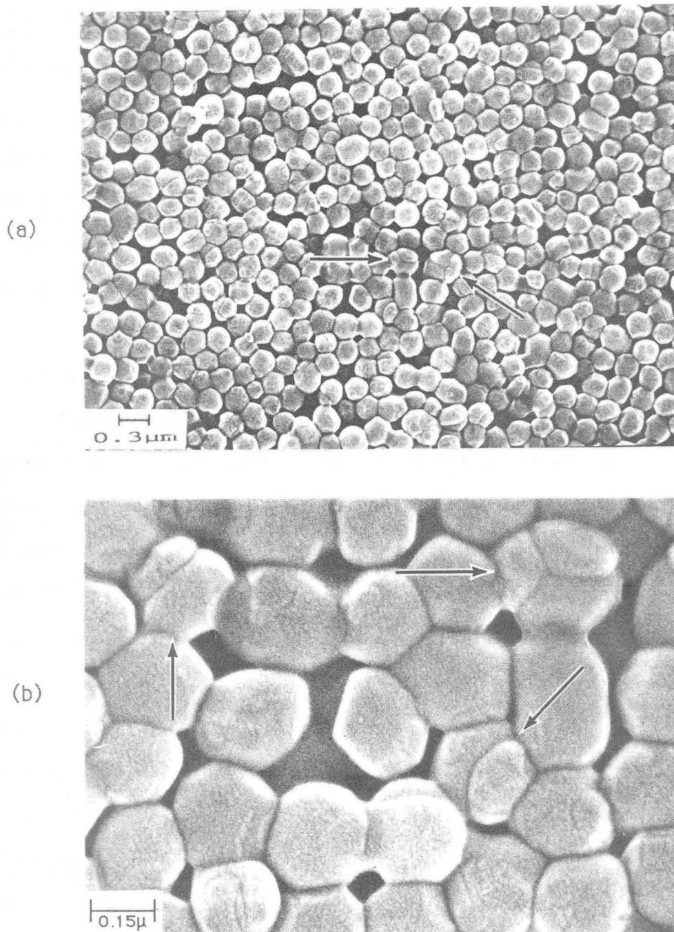
Figure 14. High magnification images of "ideal" grain structure clearly show grain boundaries within former "particles." Arrows in (a) point at a three- and a four-grained particle in the center-right portion of the micrograph. (b) Two- and three-grain particles are easily seen. Treatment: 1000°C for 1 hr.
