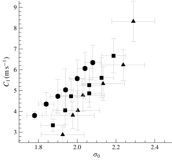
FIGURE 34. The sound speed of the bubbly mixture upstream of the shock, C_{1S} , versus cavitation number, \sigma_0 , for three inlet speeds U_0 = 6 \text{ m s}^{-1} ( \blacktriangle ), 8 \text{ m s}^{-1} ( \blacksquare ) and 10 \text{ m s}^{-1} ( \bullet ).
