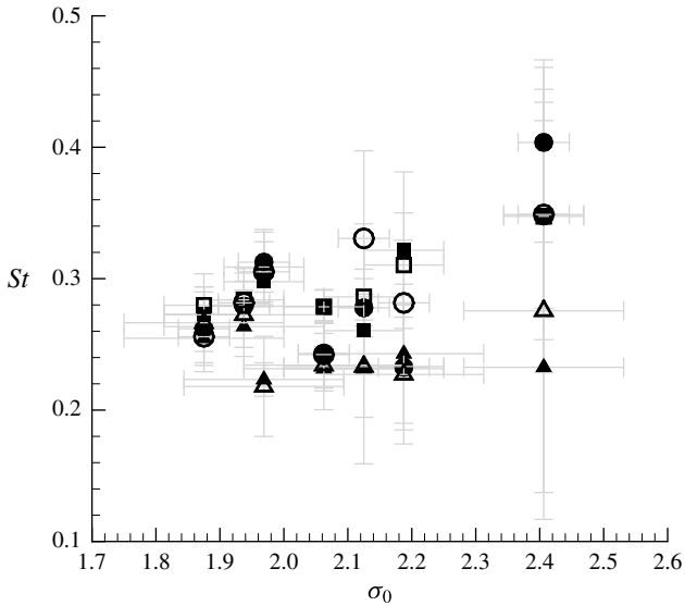
FIGURE 24. Strouhal number, St , for varying cavitation number, \sigma_0 , for three inlet speeds U_0 = 6 m s -1 ( \blacktriangle ), 8 m s -1 ( \blacksquare ) and 10 m s -1 ( \bullet ). The open symbols are data from the pressure measurements and the closed symbols are from the void-fraction measurements.
