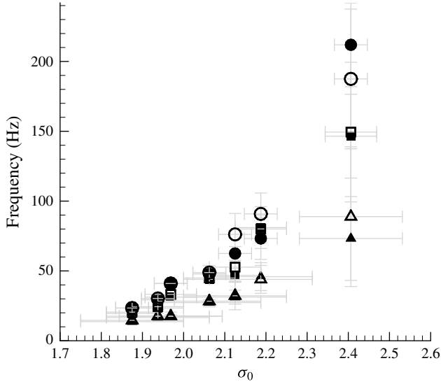
FIGURE 23. The measured dominant frequency, f , with cavitation number, \sigma_0 , for three inlet speeds U_0 = 6 m s -1 ( \blacktriangle ), 8 m s -1 ( \blacksquare ) and 10 m s -1 ( \bullet ). The open symbols are data from the pressure measurements and the closed symbols are from the void-fraction measurements.
