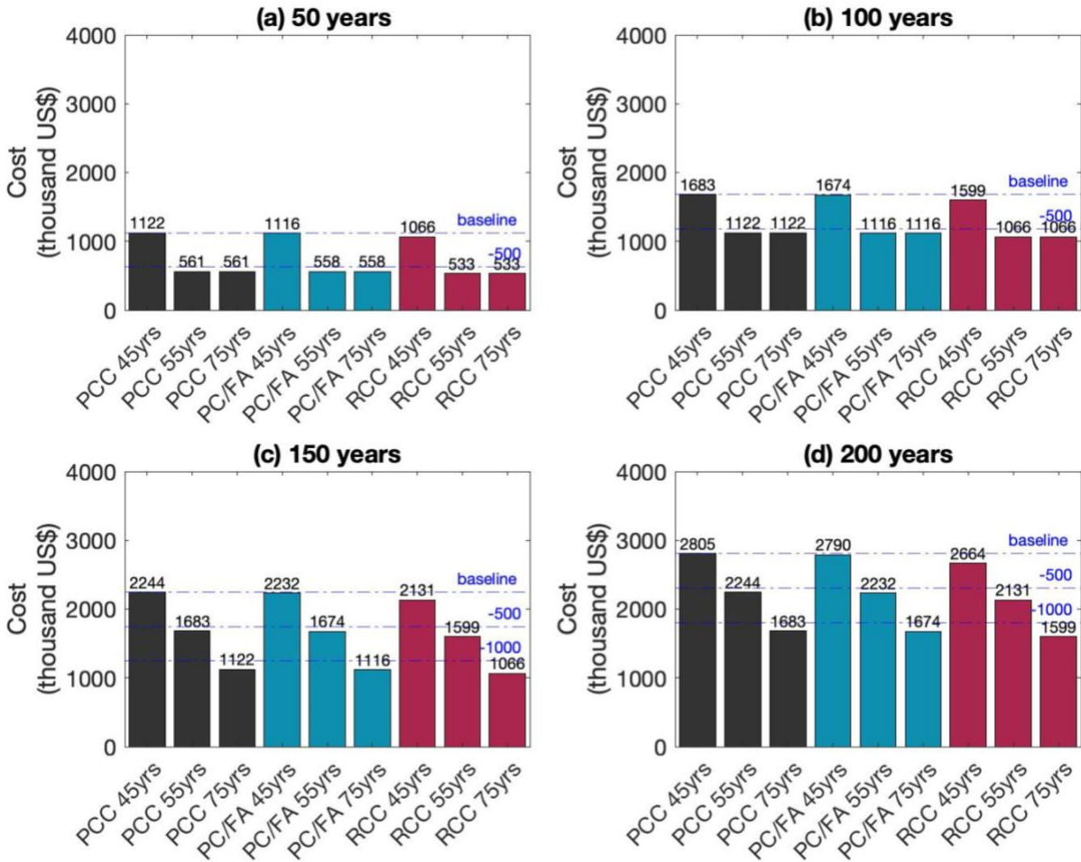
Figure 25. Costs for each PCC, PC/FA, and RCC considering 45, 55, and 75 functional lives for the pavement overlays at each of four potential service-lives of the road system, namely, 50, 100, 150, and 200 years of required service.
