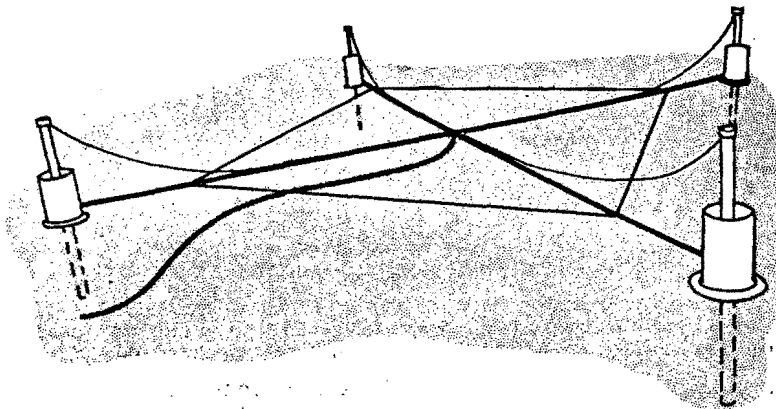
SLOPE ARRAY FOR MEASURING WAVE DIRECTION FIGURE 1
