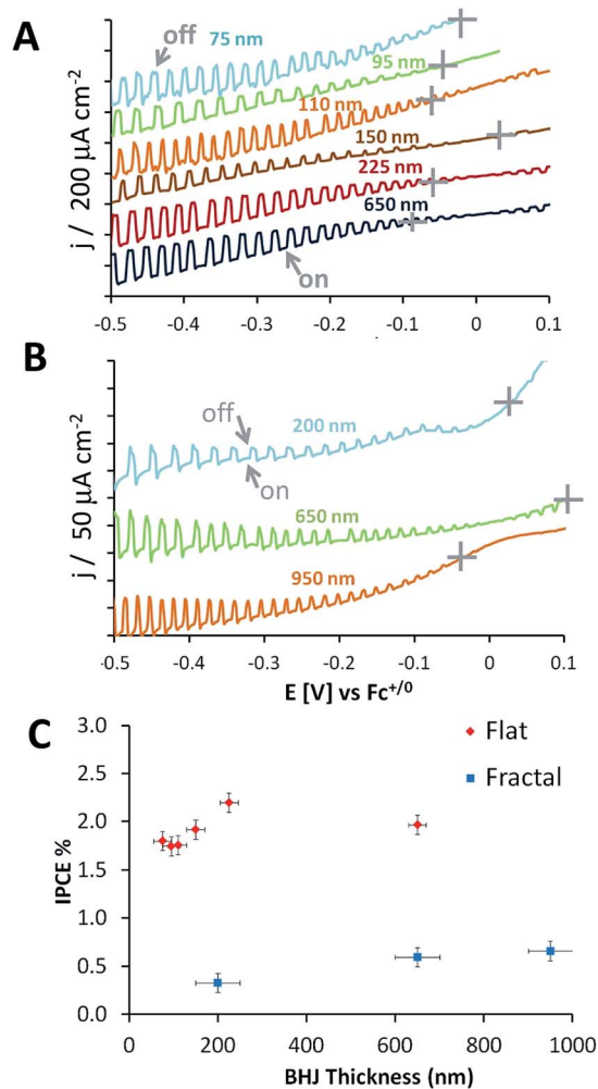
Fig. 8 Photoelectrochemical data for BHJ/PEDOT:PSS films on (A) flat and (B) fractal silver electrodes, as a function of BHJ thickness. Conditions: 0.01 M (\text{Bu}_4\text{N})\text{PF}_6 , 0.005 M \text{FcBF}_4 in \text{CH}_3\text{CN} using 435 nm LED ( 10\text{--}20 \text{ mW cm}^{-2} ). Potentials are reported versus the \text{Fc}^{+/0} potential of +0.4 V (vs. NHE). Cross-bars indicate zero current. (C) Incident photon to current efficiencies (IPCE%) versus active layer thickness.
