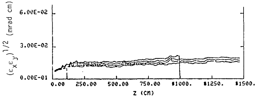
Figure 6a. Mean Transverse Emittance
