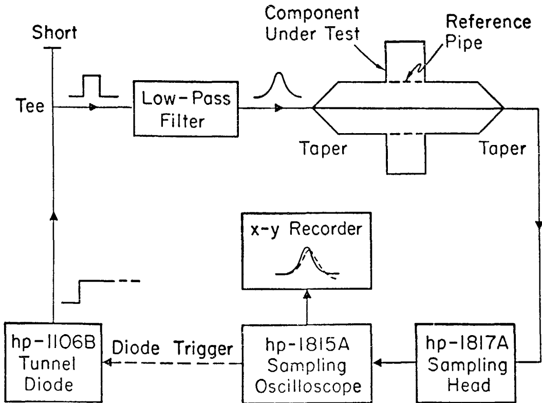
Fig. 6 -- Instrumentation for measuring t' loss parameter.
