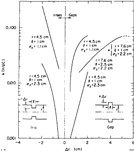
Radial gaps and irises.
