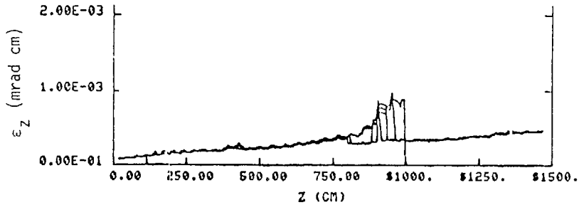
Figure 6b. Longitudinal Emittance
