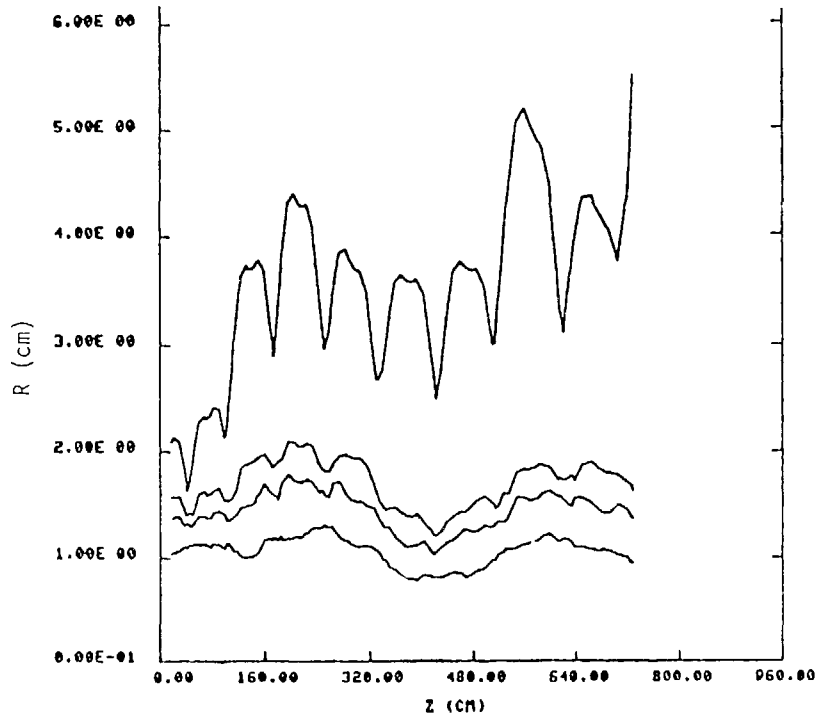
Figure 3c. Beam Radius
