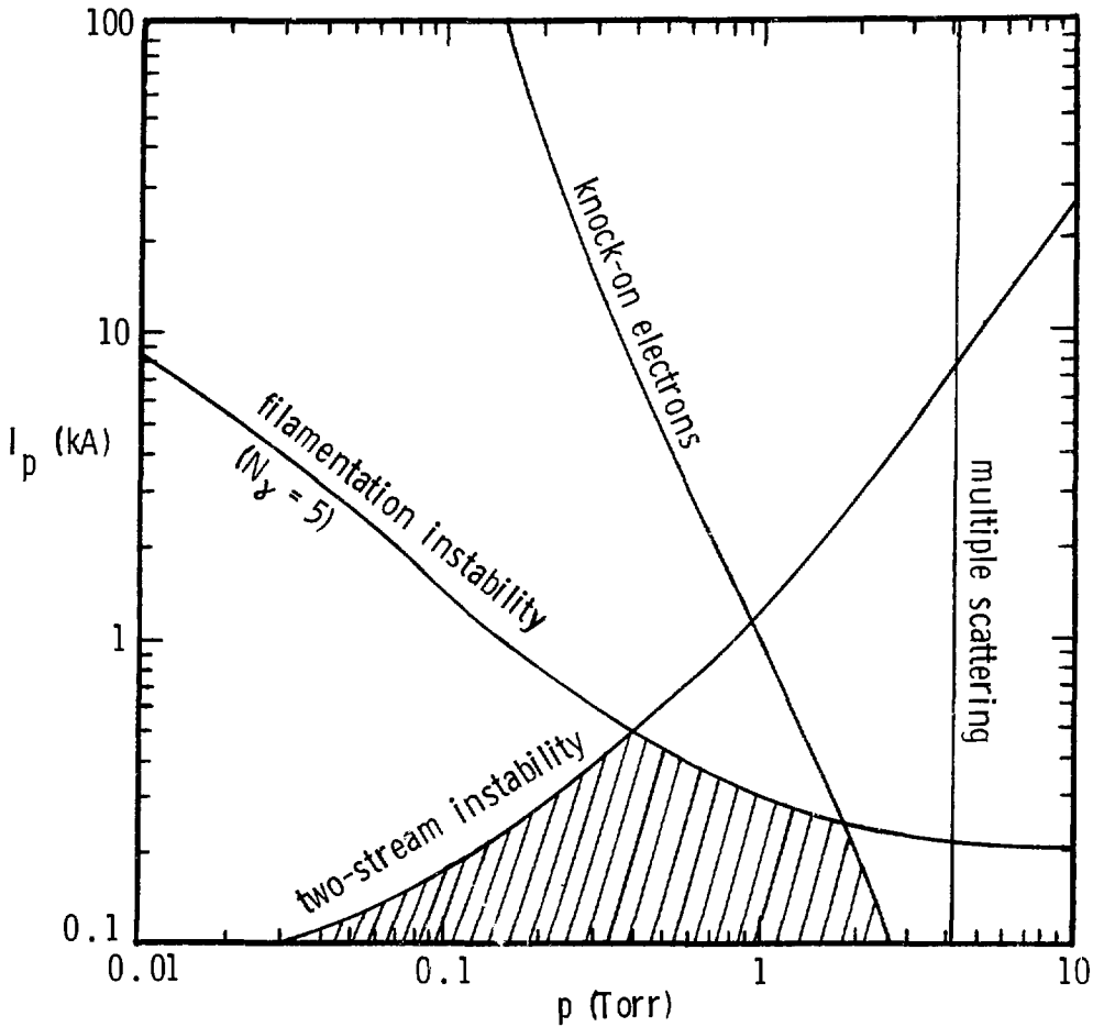
Fig. 6b. The "1 Torr window" (shown hatched) for 10 GeV uranium beam propagation in neon gas. R = 10 cm, r = 0.2 cm, L = 5 cm, T_e(r=0.2 \text{ cm}) = 100 eV, Z_{\text{gas}} = 10 , \Delta v_z/v_z = 0.005 .
