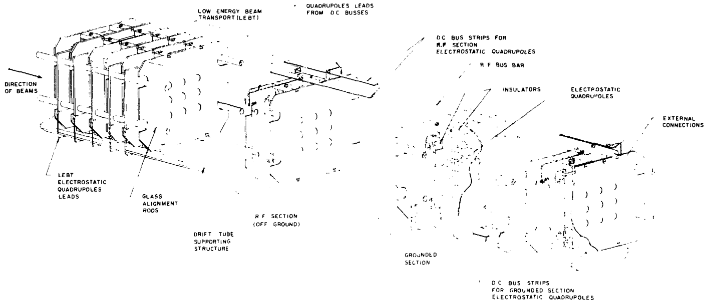
Figure 5. Schematic of M1 assembly showing bus bars. When mounted in the vacuum tank, the assembly hangs from the plate shown at the bottom.
