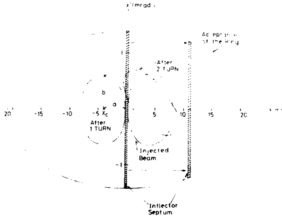
Fig. A-1 Schematic diagram of the first 2-turn-injection with the half integral tune value.
