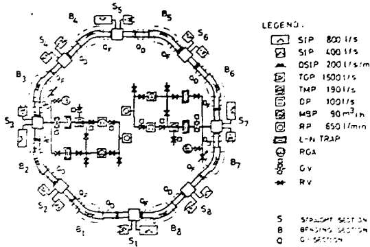
Fig.10 Vacuum System of the TARN
