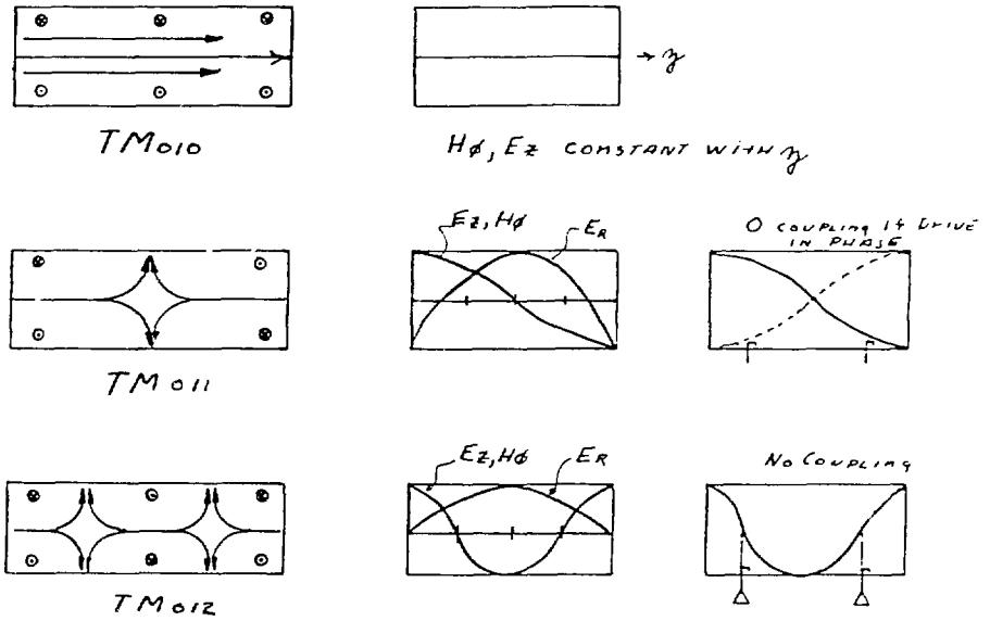
Figure 2. Field Distribution of TM_{0ln} Modes.
