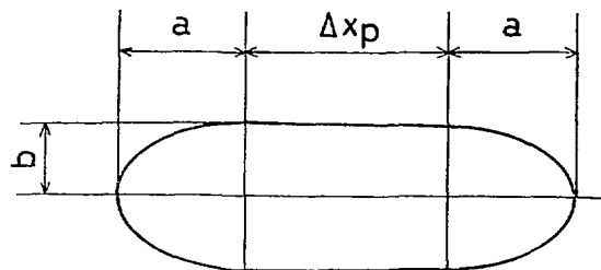
Fig. 1. The beam profile in the accumulation ring.
