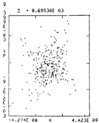
Figure 4.2. Phase-Space (x-xp) Particle Distribution
