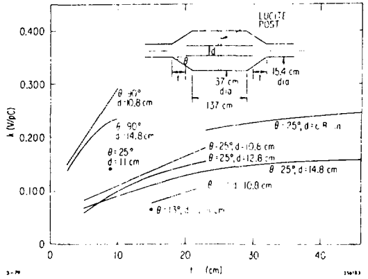
Separating plates model ( \sigma_z = 2.3 cm).
