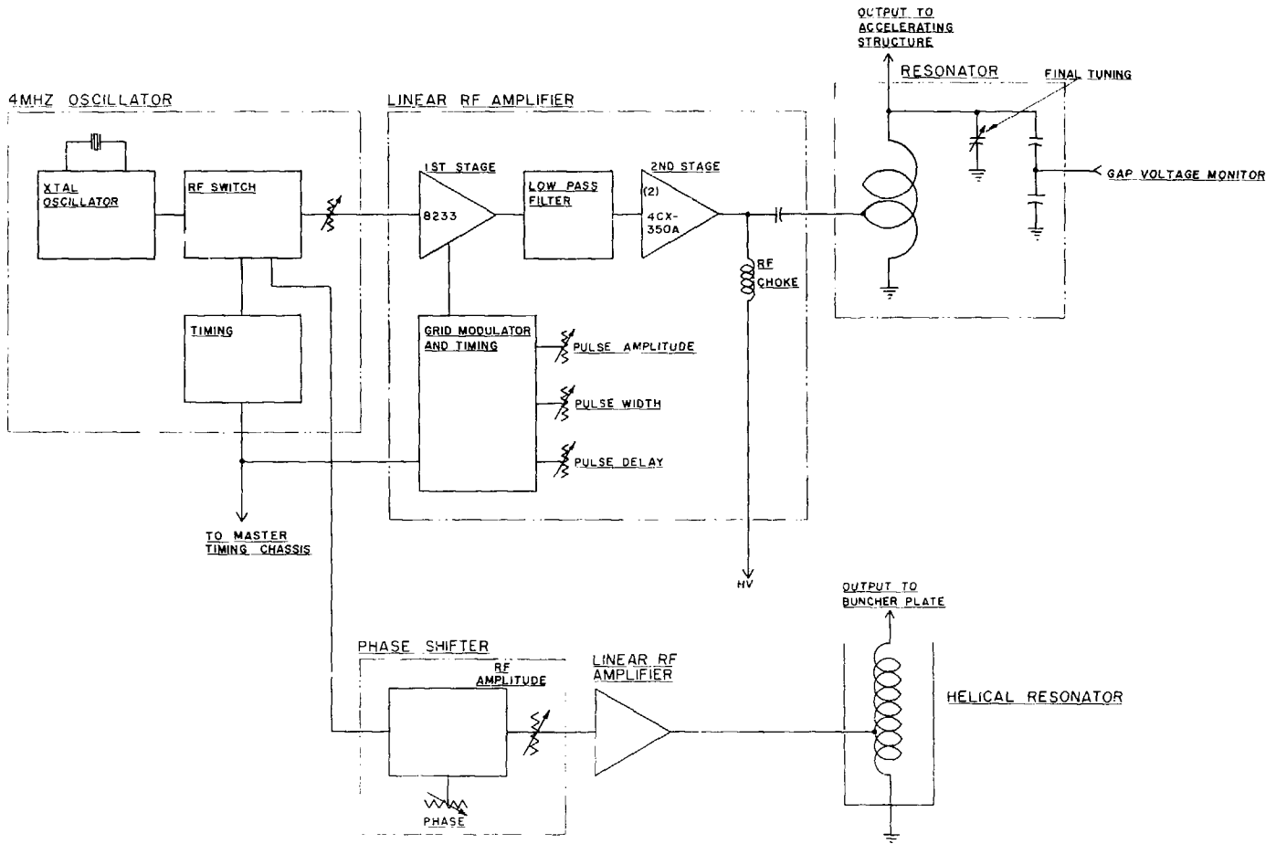
MEQALAC RF SYSTEM
