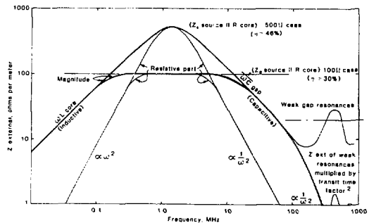
The External or Wall Impedance Part of the Coupling Impedance for (Z source Source R core)=100 \Omega /m and 500 \Omega /m Figure 6
