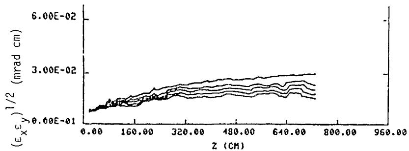
Figure 2a. Mean Transverse Emittance
