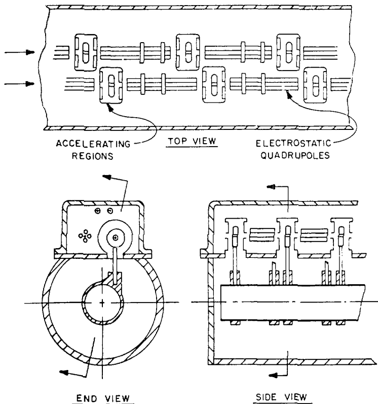
Fig. 2. Double-barreled, electrostatically focused, 311 Wideröe linac.
