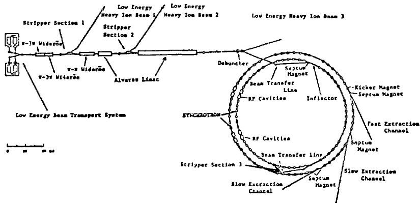
Fig. 1 Layout of NUMATRON
