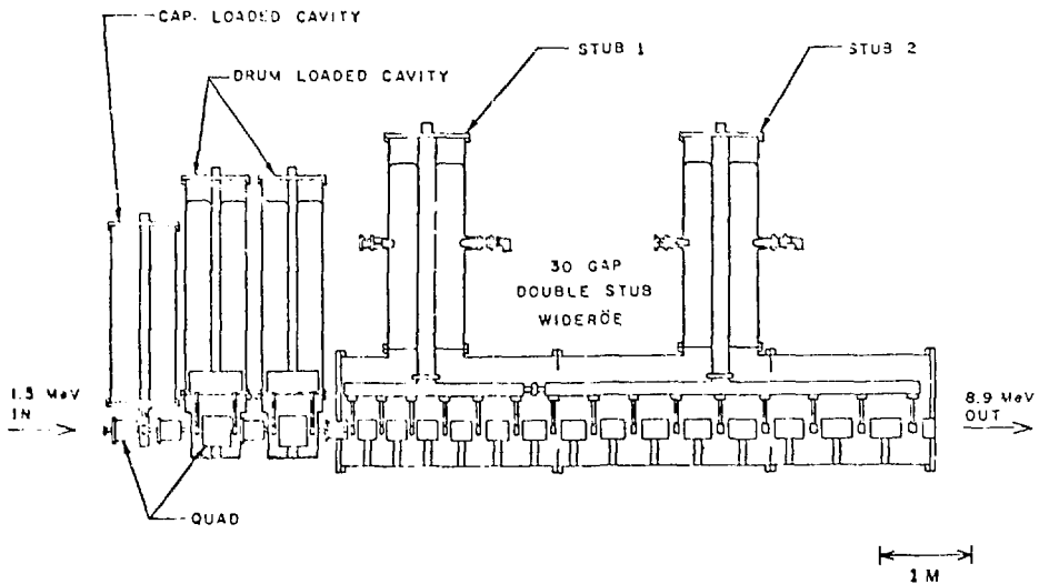
Fig. 3 30 Gap \pi/3\pi Double Stub Wideroe (Tank No. 1) and Independently-Phased Cavity Linac: 1.5 MeV to 3.84 MeV
