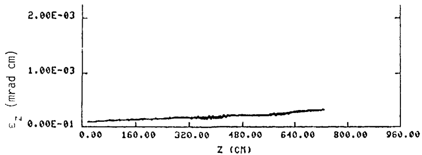
Figure 2b. Longitudinal Emittance
