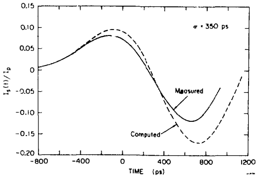
Fig. 8 -- Computed and measured functions I_s(t)/I_p for the cavity shown in Fig. 7 for a bunch length \sigma = 350 ps.
