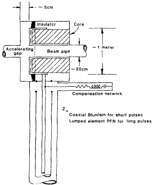
Induction Acceleration Cavity and Voltage Generator
