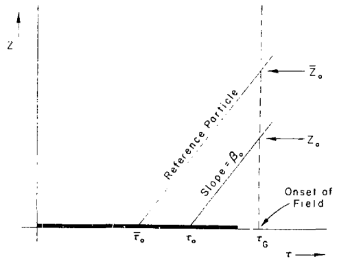
Fig. 9. Illustration of notation employed in Note 1, leading to the relation z - \bar{z} = (z - \bar{z})_0 \cdot w = \beta_0(\tau_0 - \tau_0) \cdot w .
