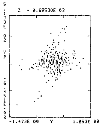
Figure 4.3. Phase-Space (y-yp) Particle Distribution
