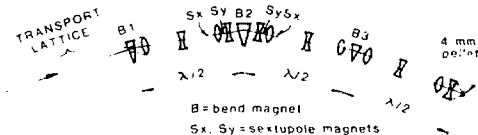
Figure 2 A 3\lambda/2 Chromatic-Correction and Matching Section
