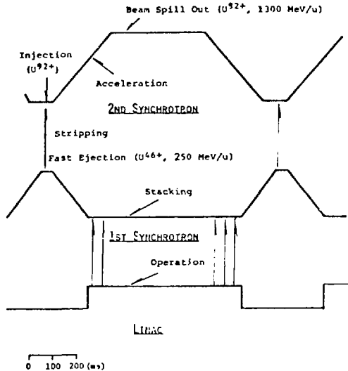
Fig.2 Operation Scheme of the Accelerator Complex
