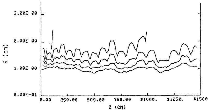
Figure 6c. Beam Radius
