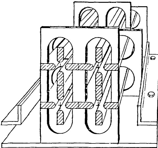
Fig. 1. Array of Four RFQ Channels
