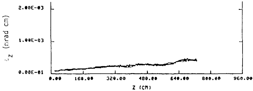
Figure 3b. Longitudinal Emittance
