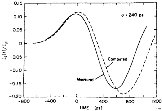
Fig. 7 -- Computed and measured functions I_s(t)/I_p for the cavity shown in Fig. 7 for a bunch length \sigma = 240 ps.
