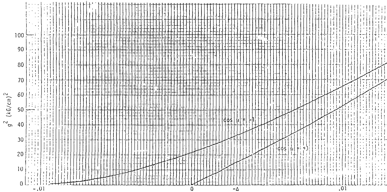
Figure 1. Magnetic Stability Limits for +-+ Geometry.
