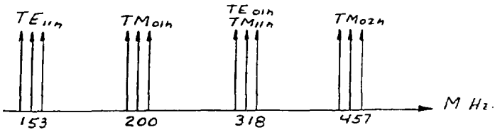
Figure 1. Modal Separation of Cylindrical Guide ( 2 = .57 Meters).
