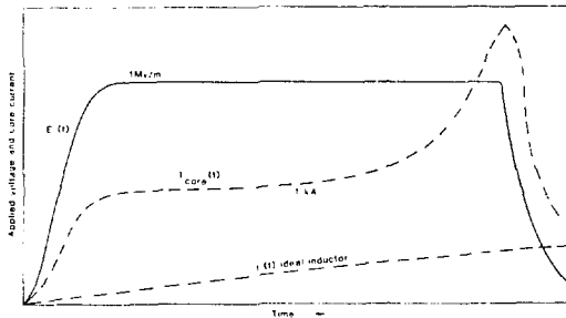
Approximate Form of Core Excitation Current
