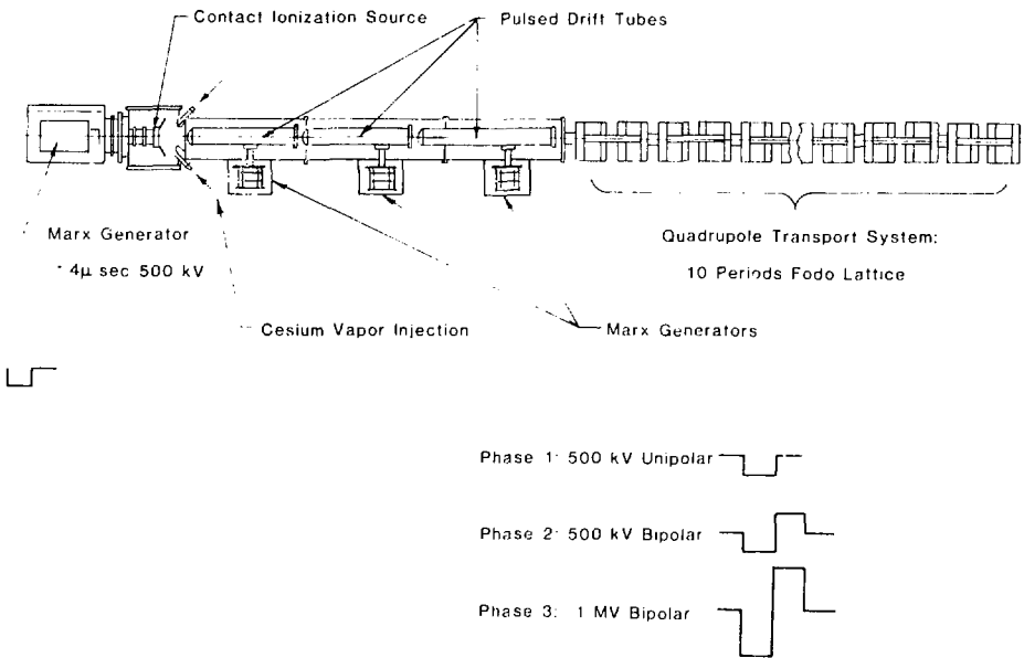
1 AMP, 2 MeV, \text{Cs}^{+1} BEAM PROPAGATION EXPERIMENT
