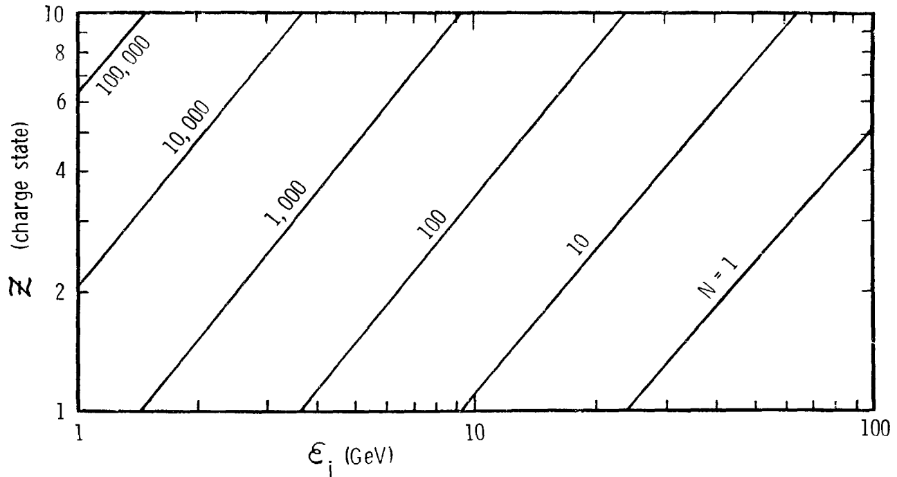
Fig. 3. Number of uranium beams ( N ) required for P = 100 TW, R = 10 cm, r = 0.2 cm, L = 10 m, A = 238 . The initial emittance was taken to be zero. For non-zero emittance, N will be larger than that shown.
