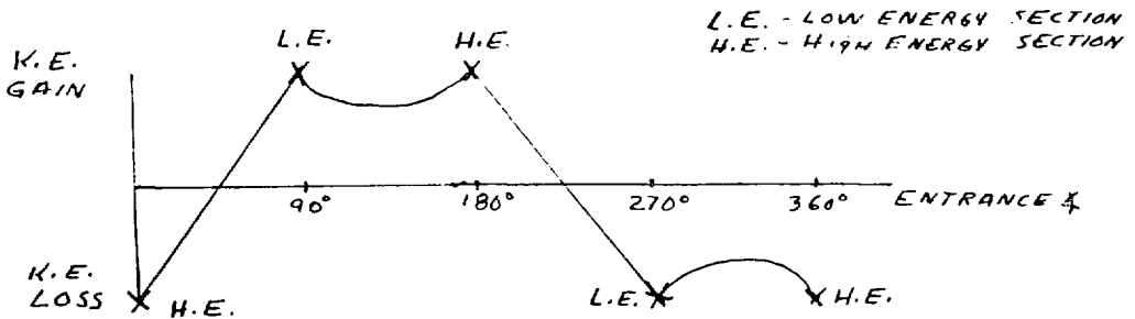
Figure 4. Velocity Change Resulting in Anti-symmetric Driving and Absorbing Function (105° Phase Advance).
