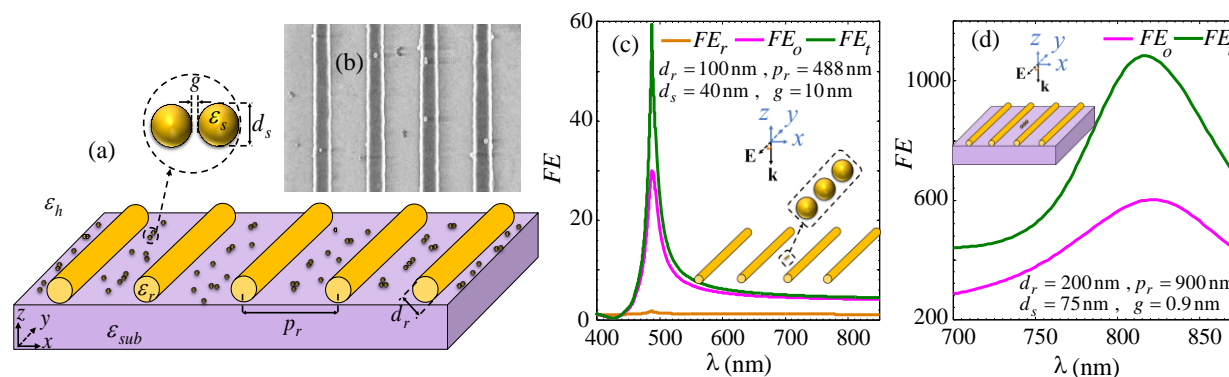
Fig. 1. (a) The schematic of the proposed two-scale structure and (b) the SEM image of the fabricated structure. The electric field enhancement versus the wavelength of incident plane wave of the two-scale structure (c) inside the vacuum host medium (d) on top of glass substrate.
