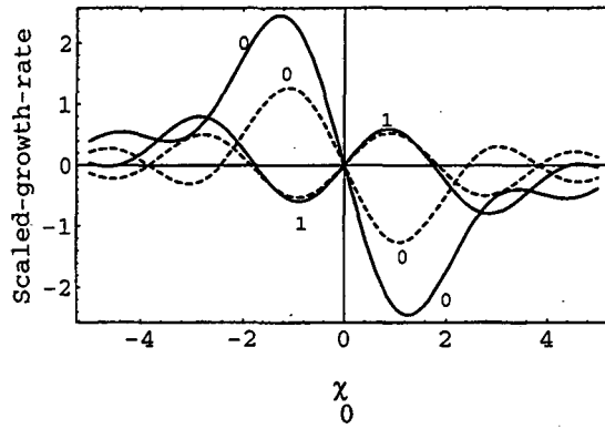
FIG. 3. Scaled growth rate, 1/\tau_s^{(l)}/\Upsilon , of a hollow beam due to the impedances of a uniform-wake (solid line) and a broadband resonator model (dashed line), when \chi_1 = 0 , \bar{z} = 0.1 . Curves are labeled by the azimuthal mode index l . See Eqs. (8) and (9) for definitions of \chi_0 , \chi_1 , and \Upsilon .
