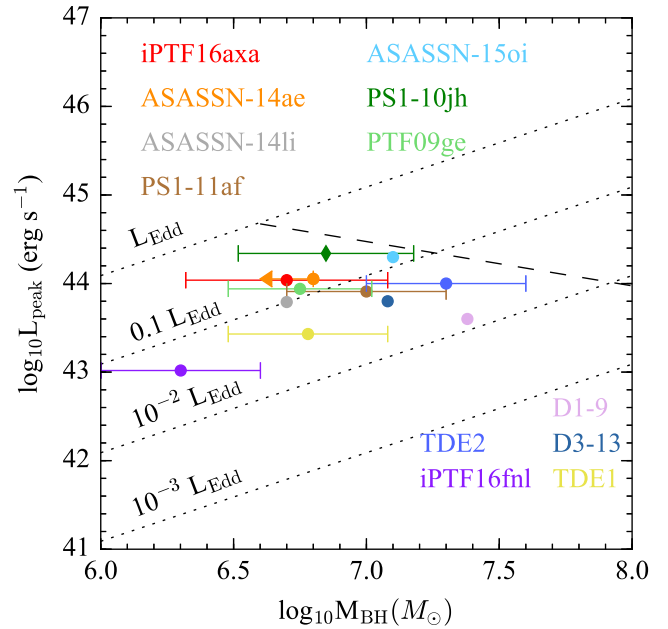
Figure 16. The peak luminosities for TDEs from Fig. 13 vs black hole masses. Black hole masses obtained from literature are marked in circles while triangles are black hole masses derived using r -band scaling in Tundo et al. (2007) . The dotted lines show the luminosities that correspond to 4 different Eddington ratios while the black dashed line shows the M_{peak} \propto M_{BH}^{-1/2} relation expected from theoretical work normalized to Eq. A1 in Guillochon & Ramirez-Ruiz (2013) with \gamma=4/3 , \beta=1 , and \epsilon=0.1 . Below M_{BH} \sim 10^{6.6} M_{\odot} , the luminosity should be Eddington-limited and scales proportionally with M_{BH} .
