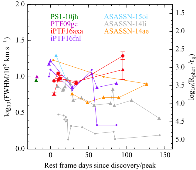
Figure 15. Comparison of the evolution of the photosphere radius inferred from emission linewidths. The triangles mark the linewidths of HeII \lambda 4686 lines while the dots mark the linewidths of H \alpha emission. The y-axis on the right hand side shows the photospheric radii in units of the gravitational radius r_g = GM/c^2 . Throughout the monitoring period, the FWHM of H \alpha and HeII \lambda 4686 line is not wider than H \alpha disfavors the scenario of a stratified BLR region that is virially bound.
