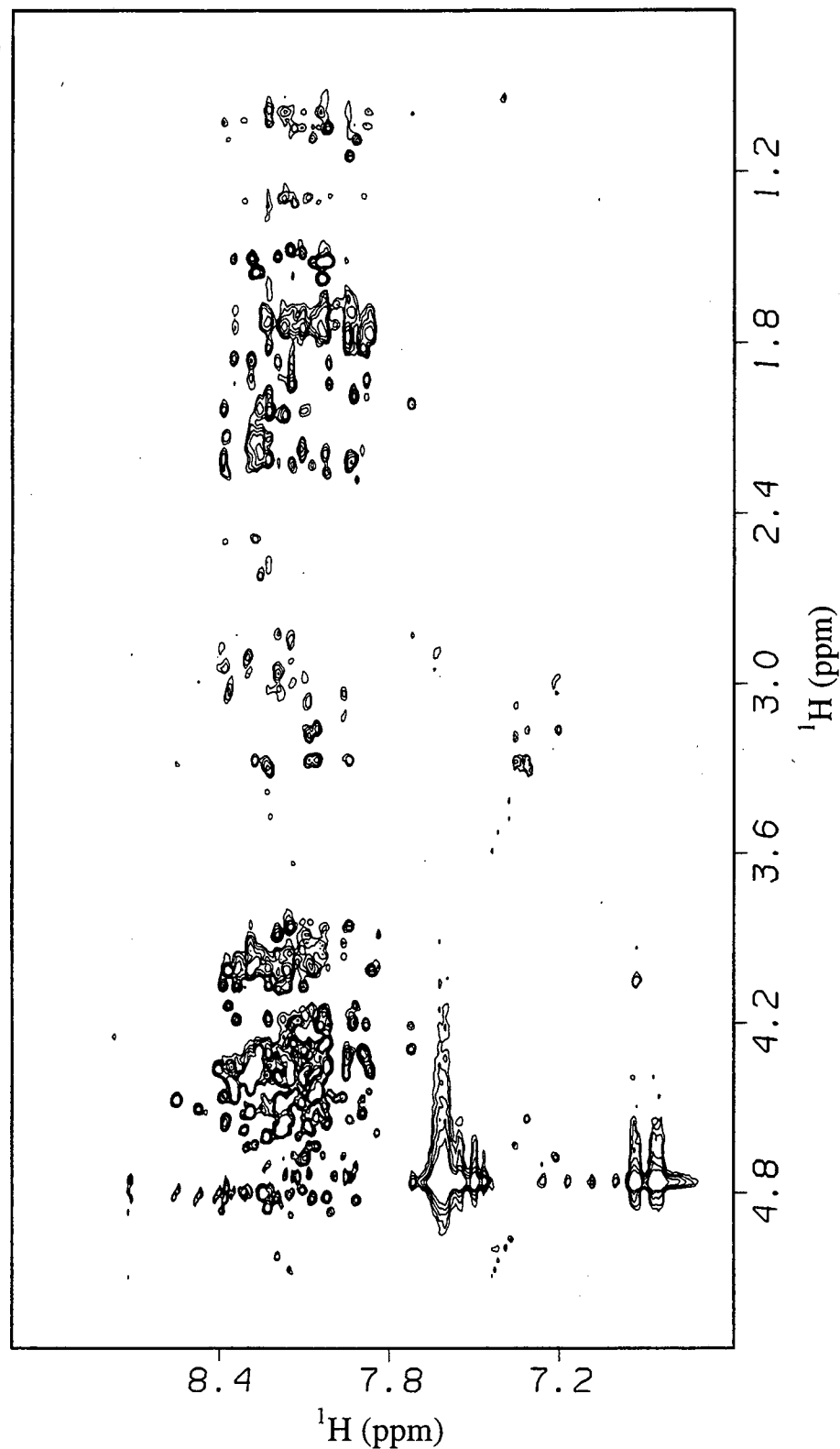
Figure 2.8C. Downfield region of a 2D NOESY experiment at 600 MHz on 271B (c-jun \delta -a1- \epsilon activation domain) at 25 °C. Protein concentration is ~0.6 mM in 70% \text{H}_2\text{O} , 10% \text{D}_2\text{O} , 20% \text{CD}_3\text{CN} , 50 mM phosphate (pH=2). The NOE mixing time is 125 ms.
