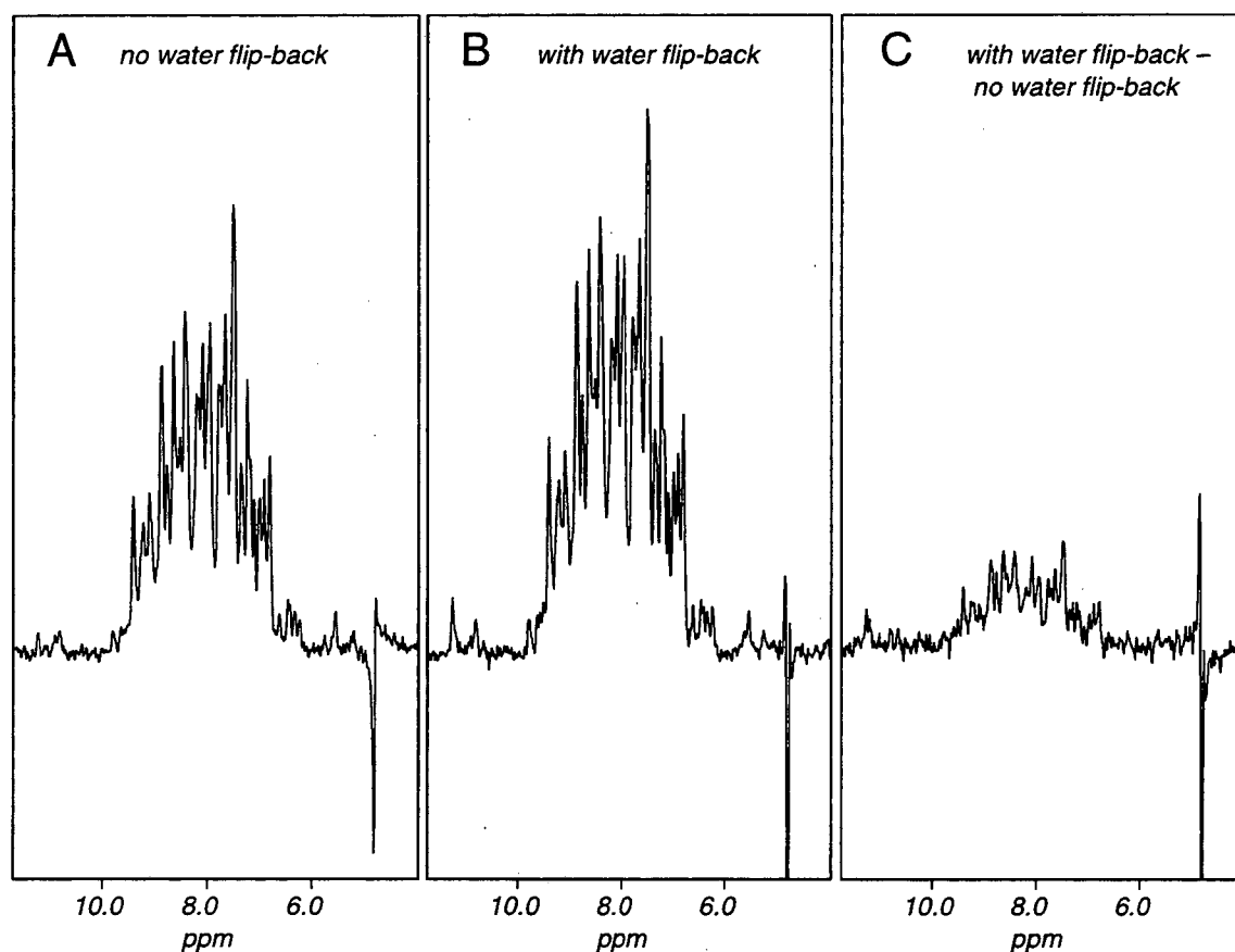
Figure 8.1. Demonstration of enhancement realized from minimal saturation of water (returning water to +Z for the recycle delay). Panel A shows the first t_1 point from an HNCO of flavodoxin (19 kD, pH=6.5) acquired with the pulse sequence in Figure 3 minus the selective water flip-back pulse. Panel B shows the corresponding "first block" obtained after inclusion of the selective water flip-back pulse immediately following the second ^1\text{H} 90^\circ pulse. Panel C illustrates the net gain in signal by subtraction of Panel A from Panel B. A gain of ~20% is observed on average, although some signals have gains of up to 100% or more.
