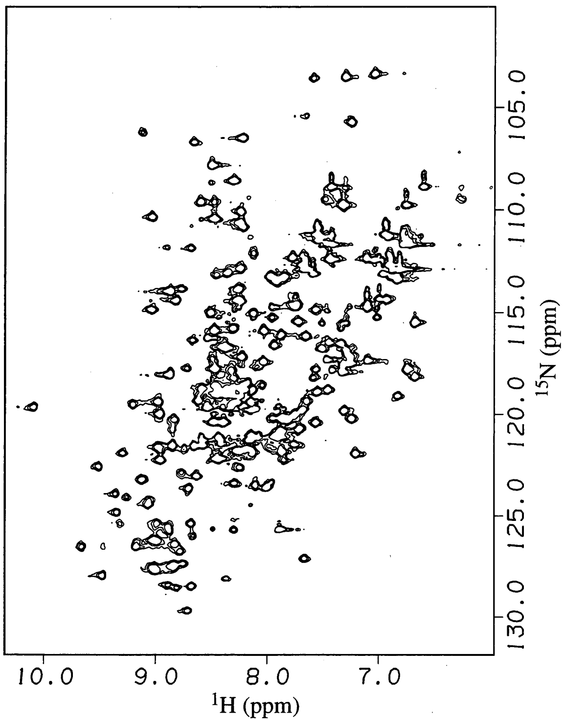
Figure 8.2A. ^{15}\text{N}/^1\text{H} HSQC (water "flip-back", sensitivity enhanced with gradient coherence selection) of RBD1+2 collected in ~2 hours at 750 MHz, 20 °C.
