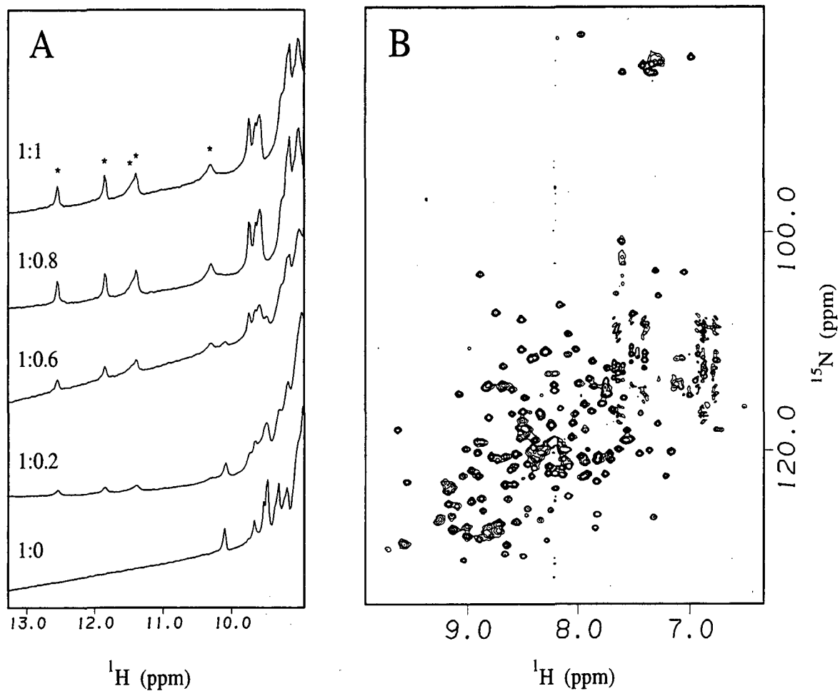
Figure 7.11. In Figure 7.11A, the 1D titration of RBD1+2 by 5'-GUUUUUUUUC-3' is shown. Imino protons are indicated by asterisks, and protein/RNA ratios are indicated for each step. In Figure 7.11B, the 600 MHz ^{15}\text{N}/^1\text{H} HMQC of RBD1+2 complexed with 1 equivalent of 5'-GUUUUUUUUC-3' is shown. Protein concentration is \sim 0.3 mM. Conditions are pH=6.5, 25 ^{\circ}\text{C} .
