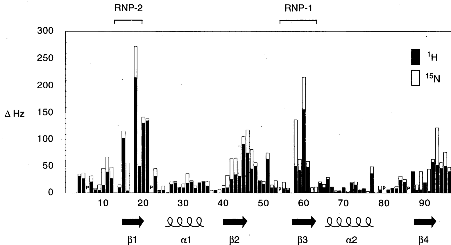
Figure 7.8. Chemical shift changes (in Hz) between RBD2 in the presence and absence of d(5' - TTTTGTTGTTTTTTTCTAG), plotted as a function of amino acid residue position. Positions labeled with P correspond to proline residues. Residue positions without chemical shift change data correspond to untrackable resonances due to intermediate exchange rates.
