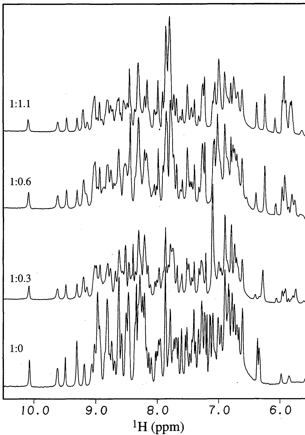
Figure 7.10. 1D titration of RBD2 with 5'-GUUUUUUUUC-3' RNA, pH = 6.0, RBD2 concentration = 1 mM. RBD2/RNA stoichiometries are shown for each titration step.
