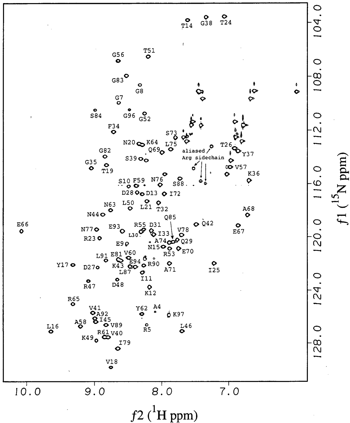
Figure 4.1. 2D HSQC ^{15}\text{N} - ^1\text{H} correlation spectrum of uniformly ^{15}\text{N} -labeled Sxl RBD-2 and assignments. Unlabeled crosspeaks between 108 and 116 ppm are NH2 groups from Asn and Gln sidechains.
