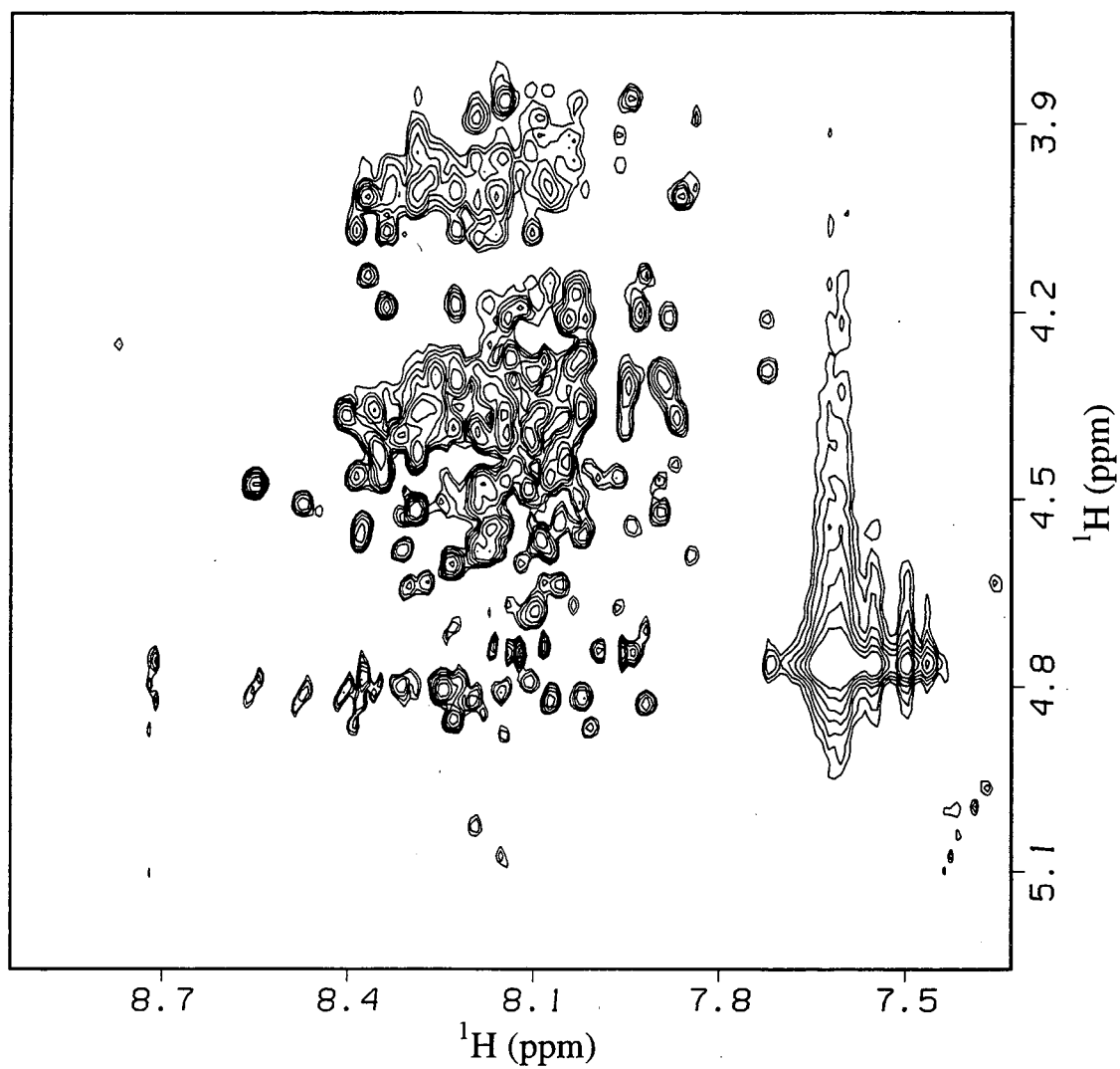
Figure 2.8B. \text{H}_\alpha -HN ("Fingerprint") region of a 2D NOESY experiment at 600 MHz on 271B (c-jun \delta -a1- \epsilon activation domain) at 25 °C. Protein concentration is ~0.6 mM in 70% \text{H}_2\text{O} , 10% \text{D}_2\text{O} , 20% \text{CD}_3\text{CN} , 50 mM phosphate (pH=2). The NOE mixing time is 125 ms.
