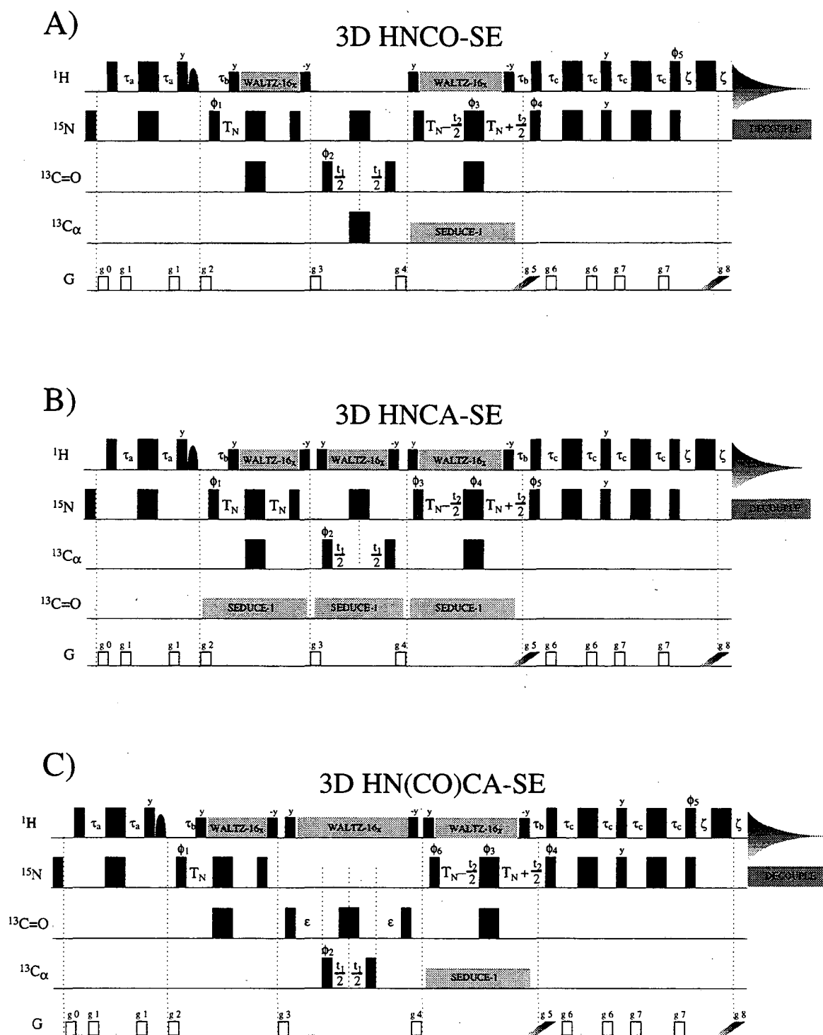
Figure 8.3. Triple resonance pulse sequences used for the assignment of RBD1+2 complexed with the Tra-PPT 10-mer. All three pulse sequences employ elements which increase overall sensitivity as discussed in the text, namely sensitivity enhancement, water flip-back pulses, and proton decoupling during remote transfer steps. A) HNCO-SE B) HNCA-SE C) HN(CO)CA-SE.
