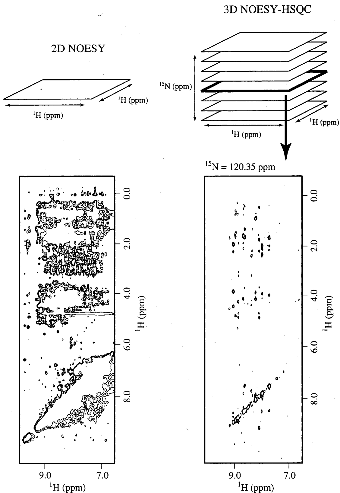
Figure 1.7. Demonstration of the resolution gains from 3D NMR. Both spectra are of a 21 kD protein (Sxl-RBD1+2) bound to RNA (5'-GUUUUUUUC-3').
