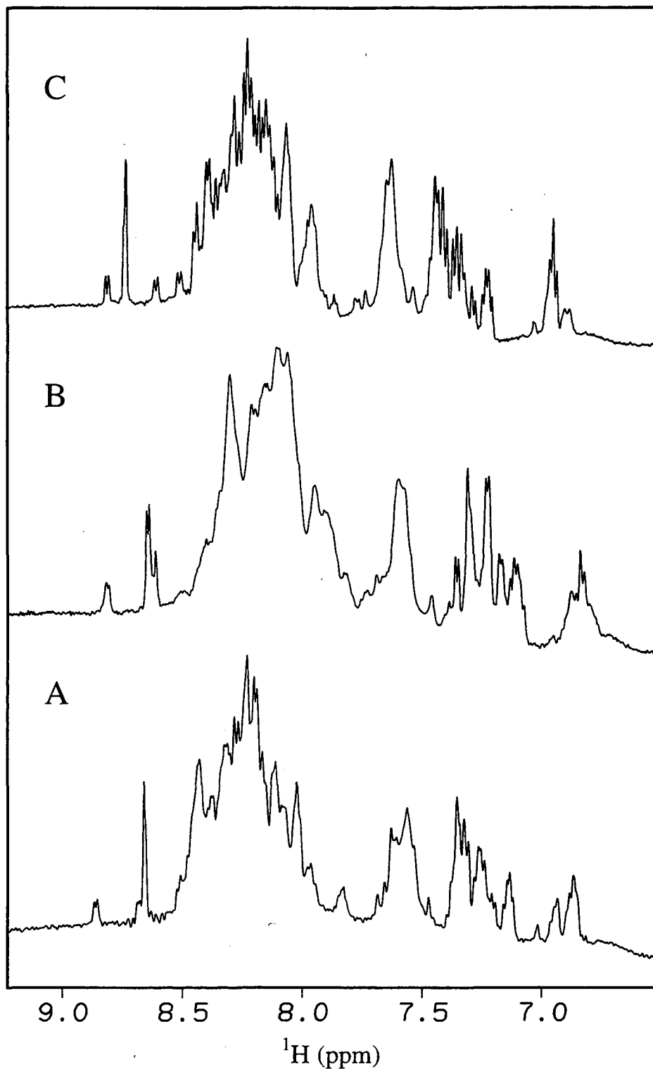
Figure 2.7. Amide and aromatic region of 1D NMR spectra at 500 MHz of 271B in various organic mixed-phase solution conditions. A) aqueous, pH=2 B) 10% trifluoroethanol (TFE), pH=2 C) 20% acetonitrile, pH=2. All spectra were acquired at 25 °C.
