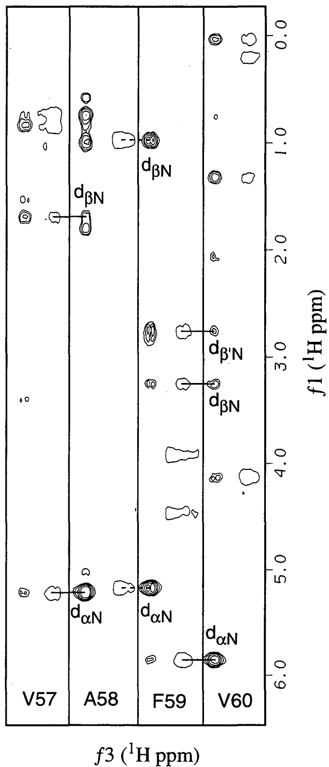
Figure 4.2A. NOESY/TOCSY strip plot. See Figure 4.2 legend on next page for a full description.
