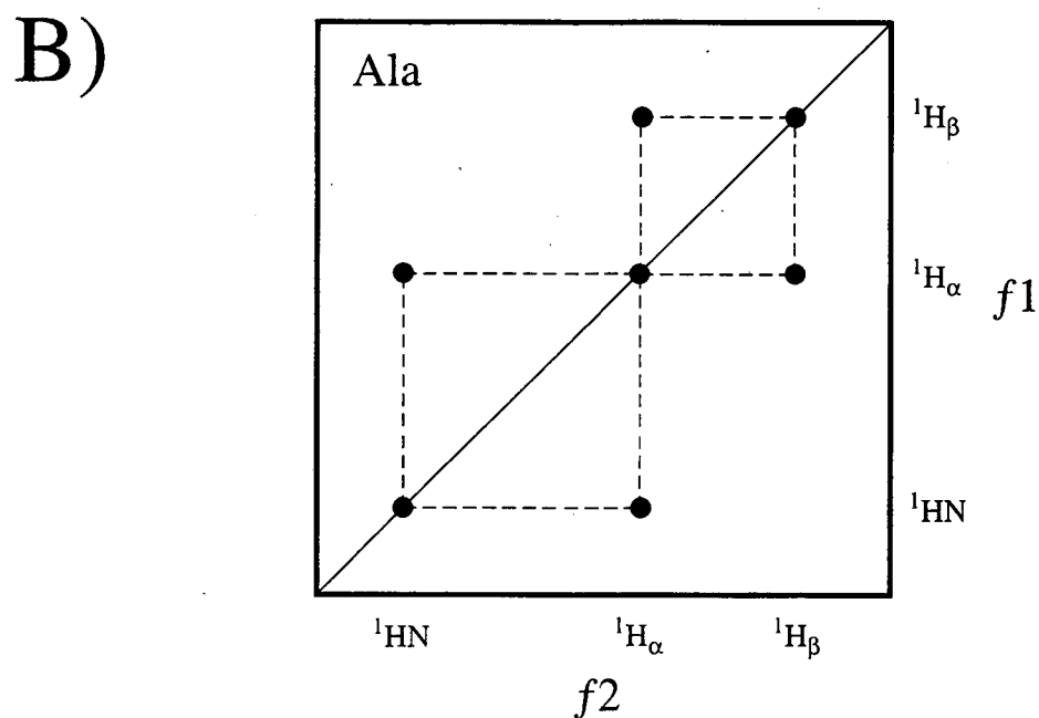
Figure 1.4. Two-dimensional COSY experiment. A) The pulse sequence is presented, and the four fundamental elements of a 2D experiment are shown. Both pulses are 90^\circ pulses. B) The resulting Fourier transformed COSY spectrum of an alanine residue. Off diagonal "peaks" correlate (dashed lines) two individual spins.
