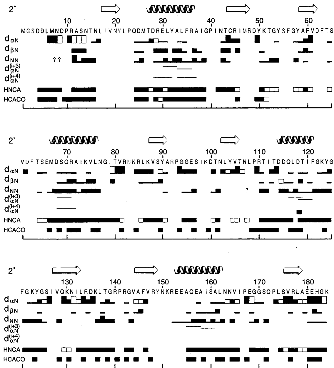
Figure 8.5. Summary of the triple resonance and NOE connectivities used to assign the backbone of bound RBD1+2. Gray letters indicate residues which were not assigned. "HNCA" is shorthand notation for sequential links made by correlating ^{13}\text{C}_{\alpha} chemical shifts from HNCA and HN(CO)CA. "HCACO" is shorthand notation for sequential links made from the full suite of triple resonance experiments (see text and Figure 8.4), where ^{13}\text{C}_{\alpha} and ^{13}\text{C}' chemical shifts were correlated simultaneously. NOE intensities are denoted by bar height as weak, medium, or strong. " d_{\beta N} " represents sequential sidechain-NH NOEs which are likely to be from beta protons. Open boxes indicate ambiguity due to chemical shift degeneracy in the case of NOEs, very weak peaks in the case HNCA/HN(CO)CA correlations, and both degeneracy and very weak peaks in the case of HCACO based correlations. Question marks denotes degeneracy in ^1\text{H} N chemical shifts.
