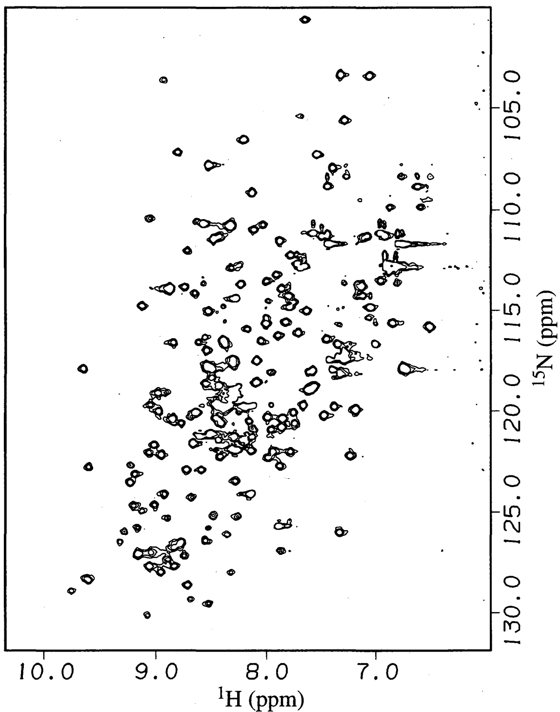
Figure 8.2B. ^{15}\text{N}/^1\text{H} HSQC (water "flip-back", sensitivity enhanced with gradient coherence selection) of RBD1+2 bound to 5'-GUUUUUUUUC-3' collected in ~2 hours at 750 MHz, 20 °C.
