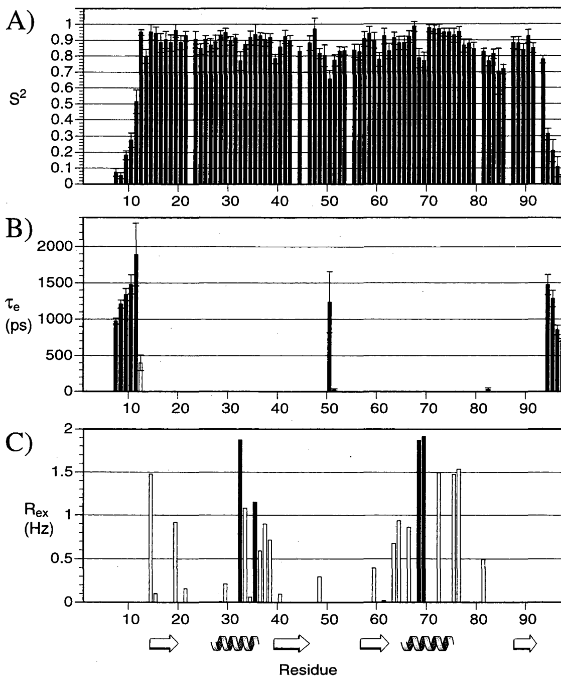
Figure 6.3. Extended Lipari and Szabo "model free" analysis of ^{15}\text{N} relaxation data in Figure 2. A) Generalized order parameter, S^2 . B) Effective or internal correlation time, \tau_e . This parameter comes from either model 2 or model 5 and is deemed significant if it is > 20 ps. Black bars correspond to \tau_e derived from model 5. White bars correspond to \tau_e derived from model 2. C) Contribution to linewidth ( = 1/\pi T_2 ), R_{ex} , from chemical exchange or other processes. Since model 4 was not used at all, all of these values are taken from the model 3 fits. Only the residues with black bars were officially ascribed an R_{ex} value for the order parameters calculated in panel A. Error bars are on the order of the values of R_{ex} .
