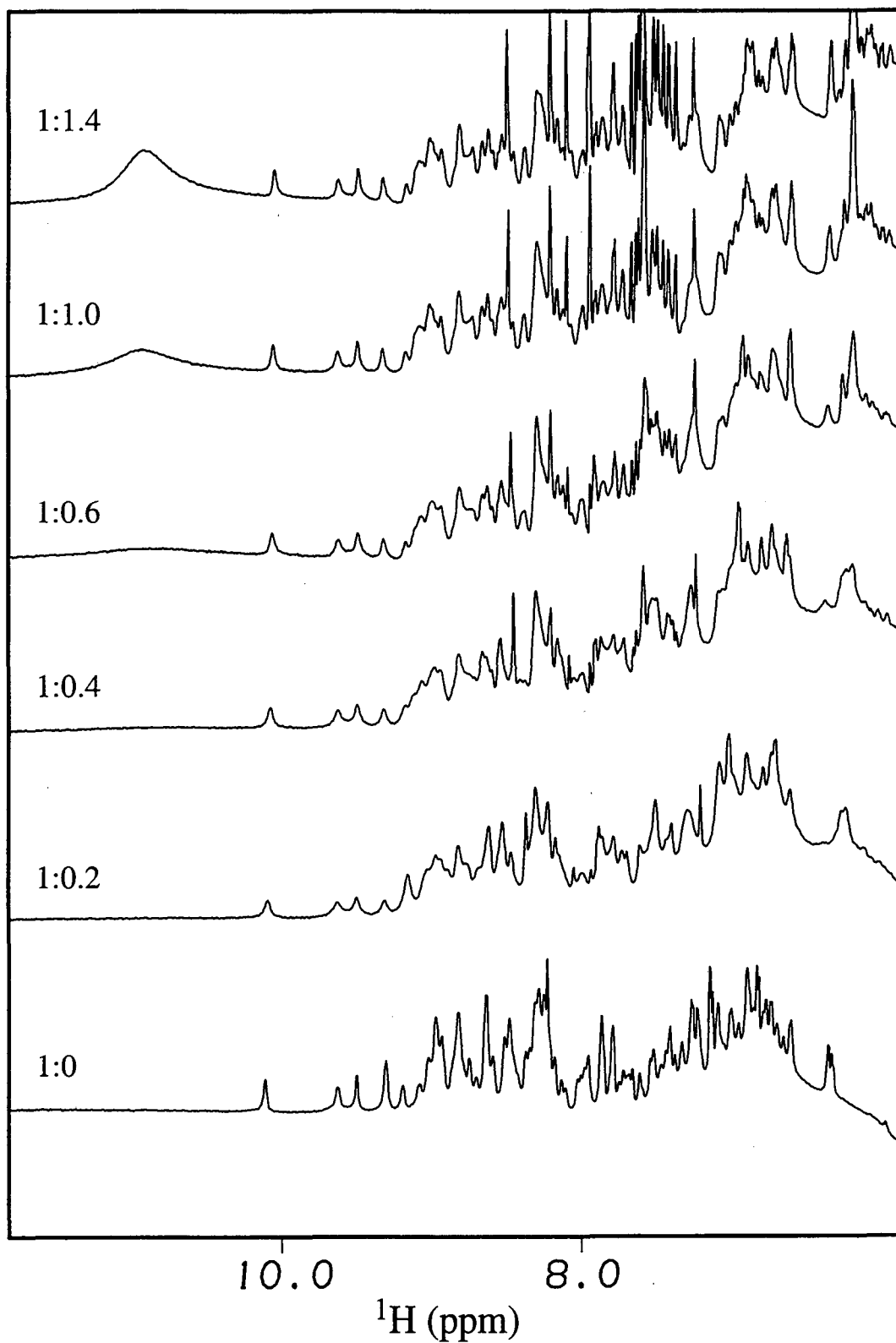
Figure 7.7. 1D Titration of RBD2 with 5'-d(TTTTGTTGTTTTTTTCTAG)-3', pH = 6.0, RBD2 concentration = 1 mM. RBD2/DNA stoichiometries are shown for each titration step.
