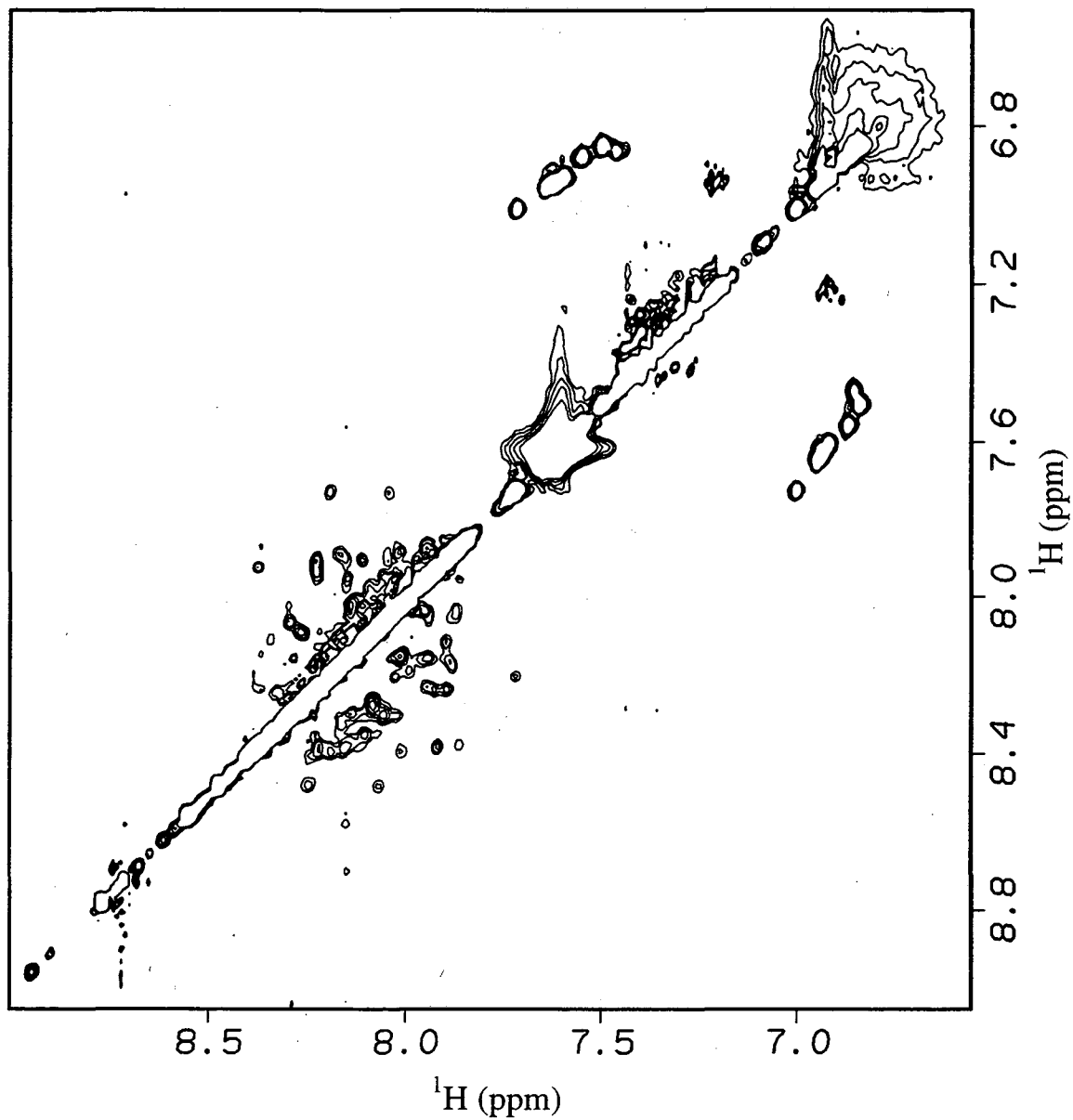
Figure 2.8A. HN-HN and aromatic region of a 2D NOESY experiment at 600 MHz on 271B (c-jun \delta -a1- \epsilon activation domain) at 25 °C. Protein concentration is ~0.6 mM in 70% \text{H}_2\text{O} , 10% \text{D}_2\text{O} , 20% \text{CD}_3\text{CN} , 50 mM phosphate (pH=2). The NOE mixing time is 125 ms.
