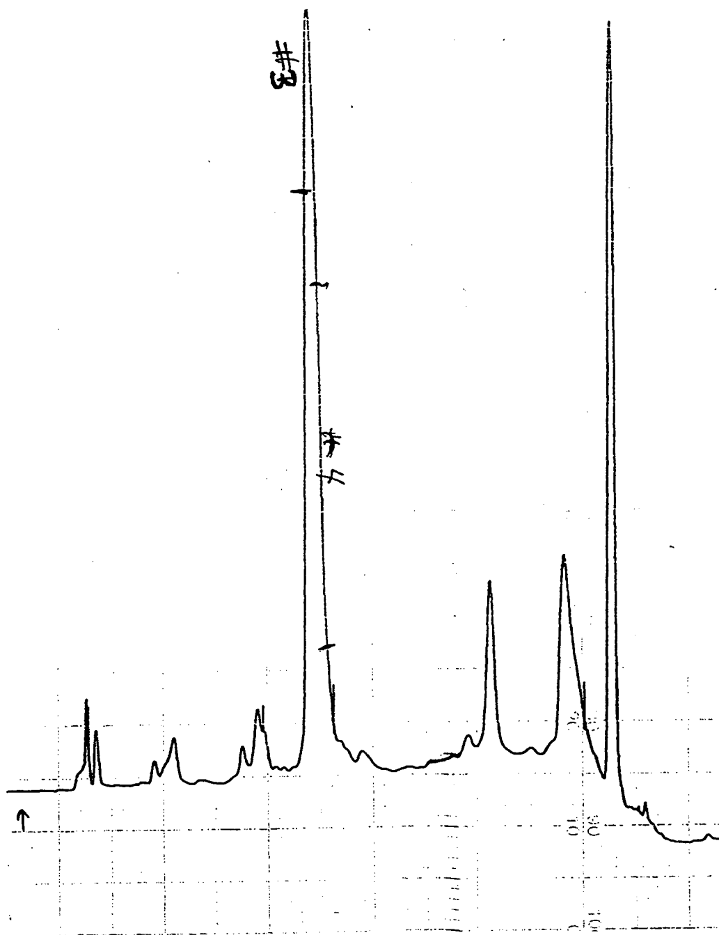
Figure 2.2. HPLC trace of the 271B purification over a reversed-phase C-18 preparative column. Approximately 7 mg was loaded for the injection shown. The run proceeds left to right. 271B elutes at the 28 minute mark, and the fractions collected are shown.
