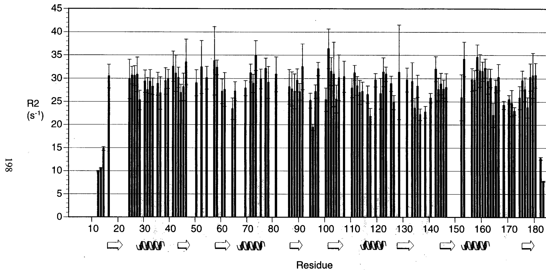
Figure 8.9. Backbone amide 15 N R2 (1/T 2 ) relaxation rates of RBD1+2 bound to the Tra-PPT 10-mer measured at 76 Mhz. Values are tabulated in Appendix B.
