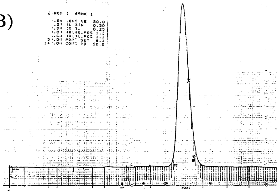
Figure 7.4. A) FPLC trace of RBD1+2 run over a Poros HS cation exchange column. The NaCl gradient is superimposed over the run. The major peak was collected in 1 mL fractions (fractions 2-6). B) FPLC trace of RBD1+2 run over a Superdex-75 gel-filtration column. The peak was collected in 1 mL fractions (fractions 24-33). The run program printout from the Pharmacia FPLC is also given.
