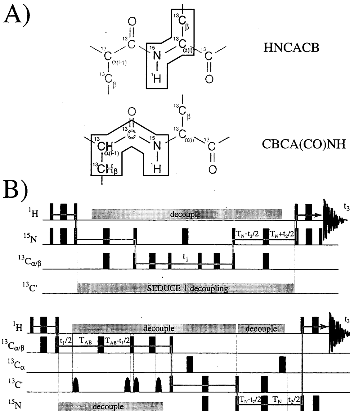
Figure 1.8. A) Schematic representation of the magnetization transfer pathways for HNCACB and CBCA(CO)NH experiments (see note in text on HNCACB additional pathway) Nuclei filled in as black are labeled by chemical shift in these experiments. B) Respective pulse sequences for HNCACB and CBCA(CO)NH. The gray line shows the path of magnetization during the course of the pulse sequences. Thin, thick, and shaped bars correspond to 90^\circ , 180^\circ , and selective 180^\circ pulses, respectively. "T" corresponds to "constant-time" periods ( T_N=12 msec).
