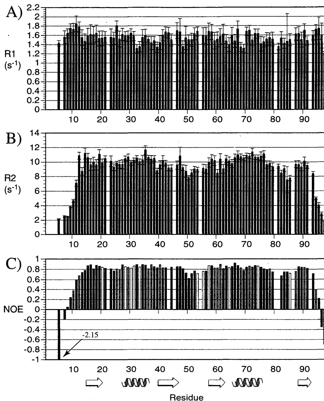
Figure 6.2. Measured ^{15}\text{N} relaxation parameters as a function of residue position for RBD2 at 25 °C, pH=5.0. A) R_1 ( 1/T_1 ) B) R_2 ( 1/T_2 ) C) ^1\text{H}/^{15}\text{N} NOE. Because the NOE experiment was collected with limited digital resolution in t_1 (80* points), there was more spectral overlap than in the T_1 or T_2 experiments (128* points). Black bars correspond to peaks with no overlap. Grey bars correspond to peaks with a slight degree of overlap. White bars correspond to peaks with a significant degree of overlap. Error bars for the NOE experiment were estimated to be 0.05 for the model free analysis.
