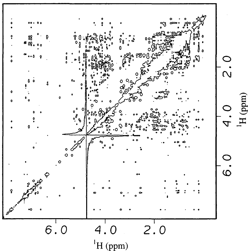
Figure 1.5. Two-dimensional ^1\text{H} - ^1\text{H} NOESY experiment. The NOESY spectrum shown is of an 11 kD protein (Sxl-RBD2) in \text{D}_2\text{O} buffer.
