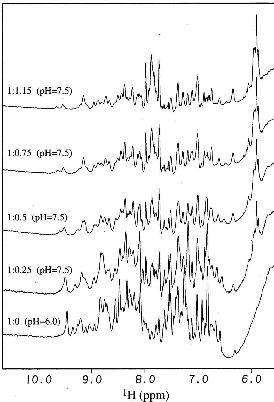
Figure 7.9. 1D titration of RBD1 with 5'-GUUUUUUUC-3' RNA, pH = 6.0, RBD1 concentration = ~0.8 mM. RBD1/DNA stoichiometries are shown for each titration step. The pH was increased to 7.5 for the second titration point.
