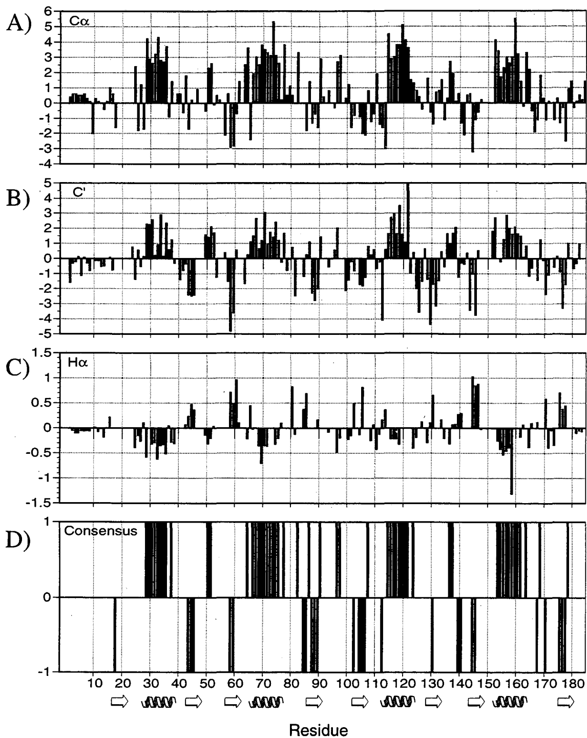
Figure 8.6. A) ^{13}\text{C}_\alpha chemical shift differences from random coil values. B) ^{13}\text{C}' chemical shift differences from random coil values. C) ^1\text{H}_\alpha chemical shift differences from random coil values. D) "Consensus" chemical shift index (CSI) as discussed in the text.
