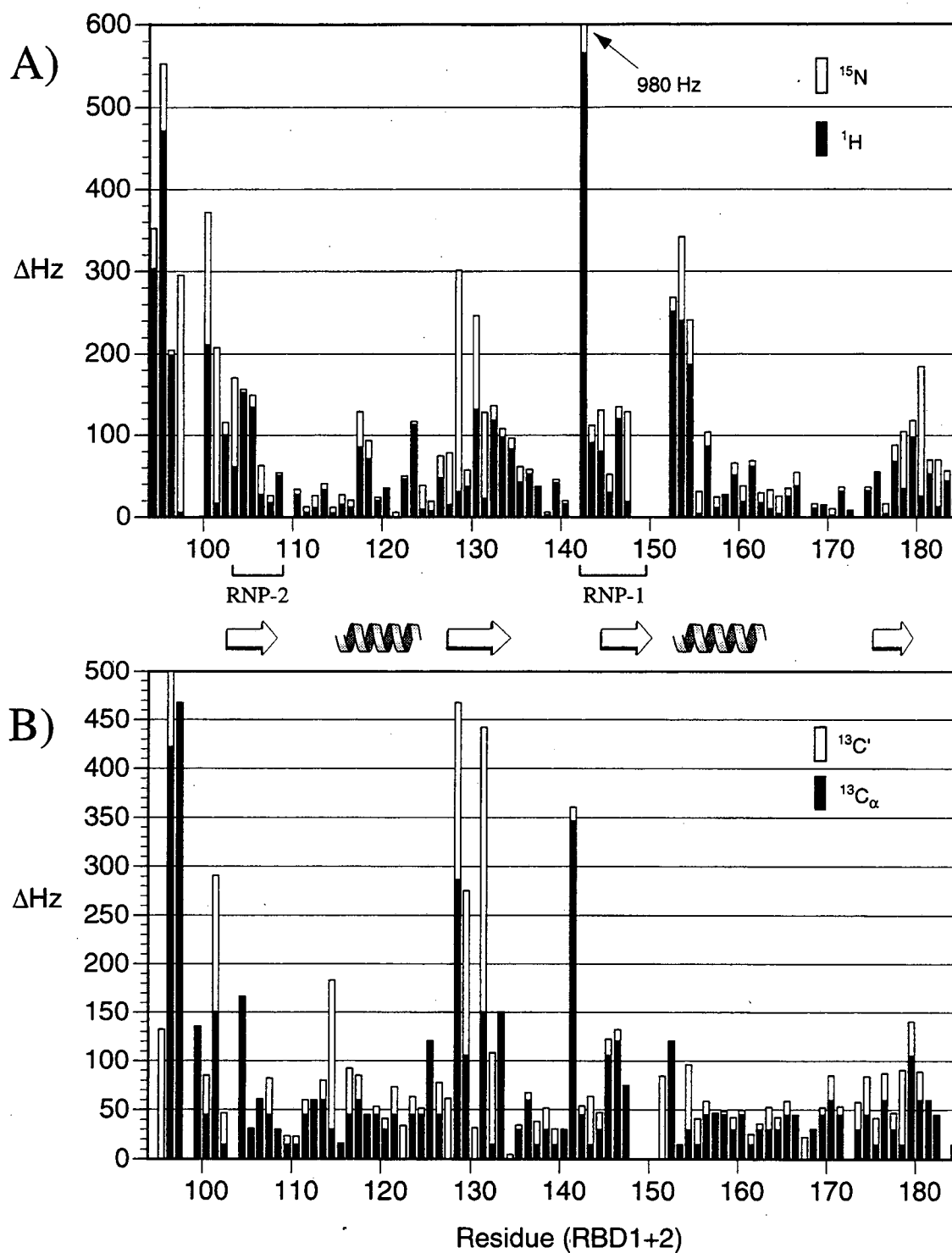
Figure 8.7. A) ^1\text{H} N (black bars) and ^{15}\text{N} (white bars) chemical shift differences between RBD1+2 bound to 5'-GUUUUUUUUC-3' and RBD2 (Chapter 4). B) ^{13}\text{C}_\alpha (black bars) and ^{13}\text{C}' (white bars) chemical shift differences between RBD1+2 bound to 5'-GUUUUUUUUC-3' and RBD2 (Chapter 4). Differences in Hz are calculated using 600 Hz/ppm. Shifts are stacked to show total shifts in Hz.
