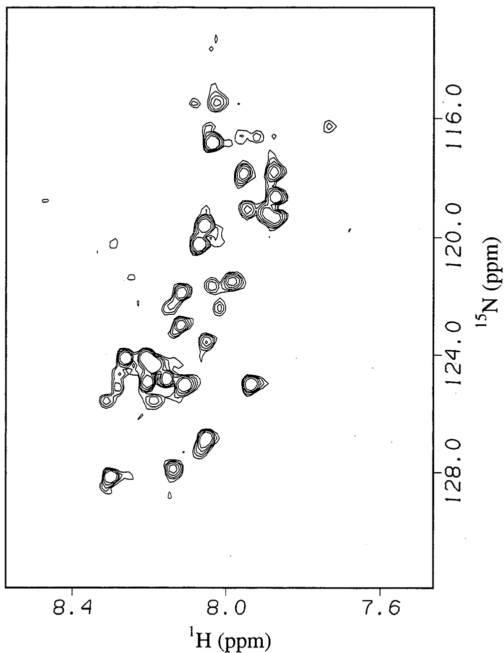
Figure 2.9. ^{15}\text{N}/^1\text{H} HSQC at 600 MHz of 0.3-0.4 mM 271B (pH=2.5) specifically labeled with ^{15}\text{N} alanine and leucine residues. 50* ( t_1 ) x 512* ( t_2 ) points were acquired over approximately 80-90 minutes (32 scans/block). The ^{15}\text{N} spectral width is 1200 Hz. The contour level multiplier for the plot shown is set at 1.5.
