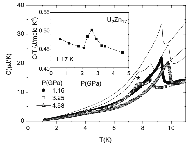
Figure 4. The specific heat of \text{U}_2\text{Zn}_{17} at three pressures (symbols). The asterisk (*) labels the transition between two magnetic phases at 3.25 GPa. Fine lines show the specific heat of \text{U}_2\text{Zn}_{17} before subtraction of addenda. The inset shows the pressure dependence of \gamma = C/T at 1.17 K.
