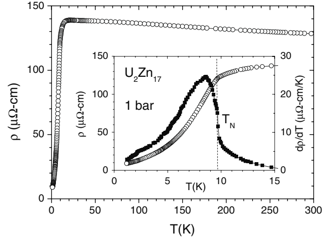
Figure 1. Electrical resistivity of \text{U}_2\text{Zn}_{17} at atmospheric pressure showing a pronounced drop of resistivity at the magnetic ordering temperature T_N . The inset compares the temperature derivative of the resistivity to the Néel temperature (vertical dashed line) determined by adiabatic specific heat.
