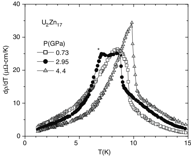
Figure 2. Dependences of d\rho/dT of \text{U}_2\text{Zn}_{17} on temperature near its magnetic transitions at representative pressures. The asterisk (*) indicates the transition between two magnetic phases at 2.95 GPa.
