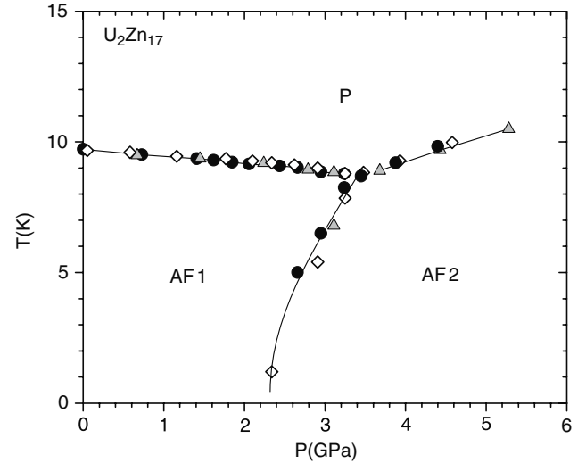
Figure 3. Magnetic pressure–temperature phase diagram of \text{U}_2\text{Zn}_{17} . The results of two resistivity experiments are shown by triangles and circles and the results of ac-calorimetry measurements are labeled by open diamonds.
