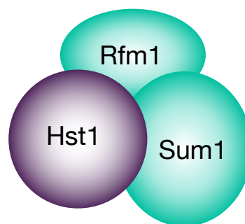
Hst1-Sum1 complex
