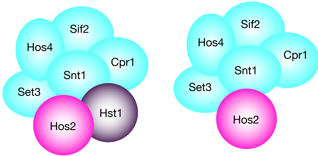
Set3 complex
