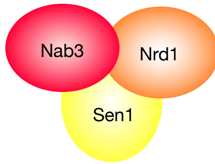
Nrd1 complex
