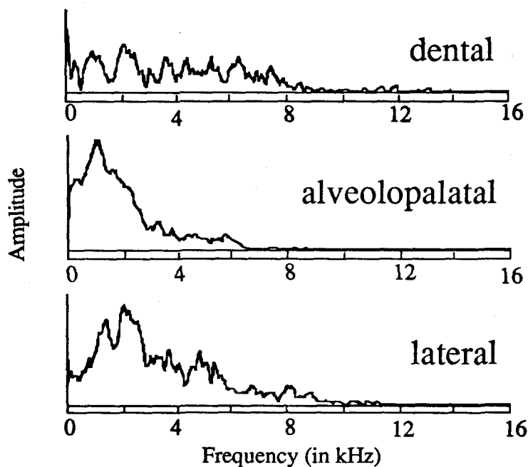
Figure 7: Mean spectra of the dental, alveolopalatal and lateral voiceless unaspirated clicks before the vowels /i,e,a/ for two male Xhosa speakers. Each curve is the mean of six spectra. Spectra were averaged over only two speakers so dissimilar tokens were not averaged together.
