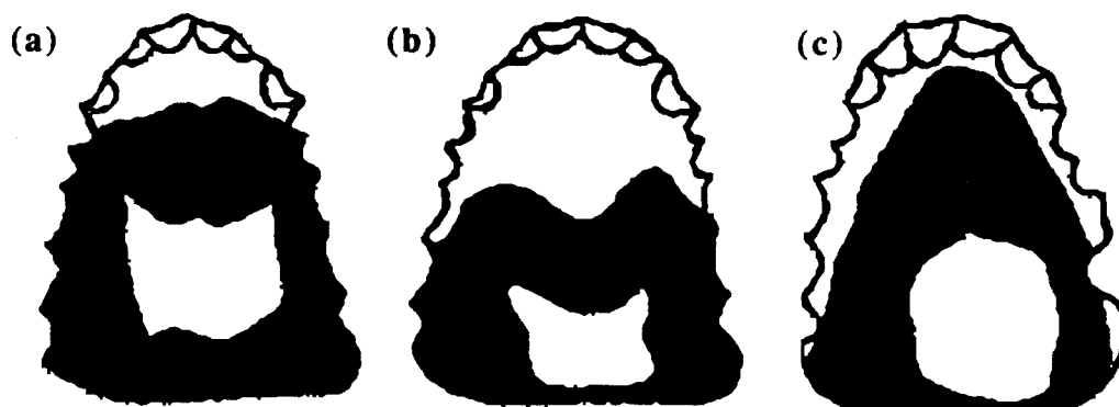
Figure 2: Palatograms of Xhosa clicks based on Beach (1938): (a) post-alveolar /!/, (b) "cerebral" /!/, (c) bilaterally released /!/. Areas of contact between the tongue and the palate are indicated by dark shading.
