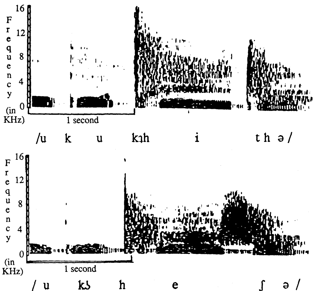
Figure 16: Wideband spectrograms of words containing voiceless aspirated dental and lateral clicks uttered by a male Xhosa speaker.
