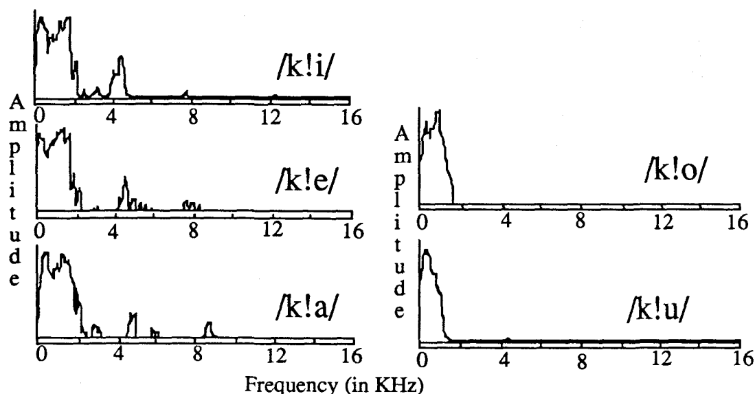
Figure 9: Spectra of voiceless unaspirated alveolopalatal clicks of one female speaker of Xhosa, before each of the five vowels.
