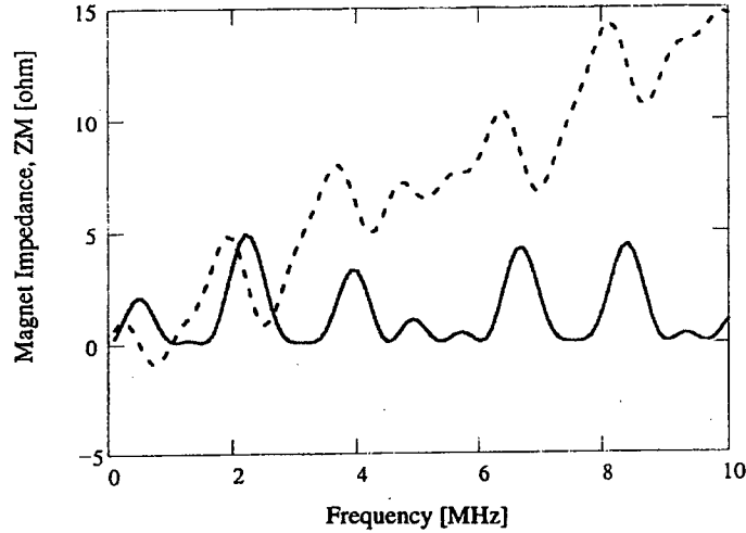
Figure 4: Impedance of the magnet. Solid — ReZ_M [ohm]. Dashed — ImZ_M [ohm].
