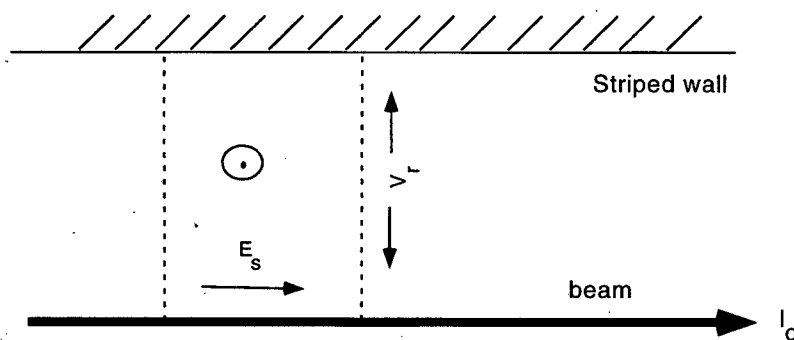
Figure 9: Fields between beam current and wall
