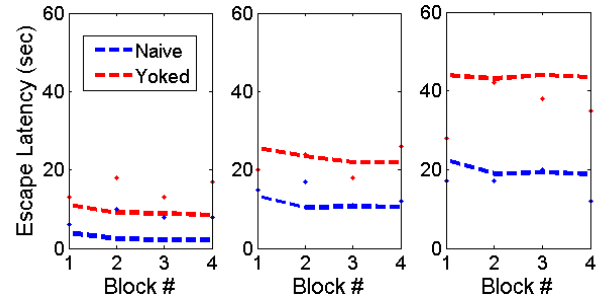
Figure 7: Simulation of the experiment by [19]. Dashed lines are model predictions; diamonds are data points. The three columns correspond to the experimental conditions requiring 1, 2, or 3 lever presses.
