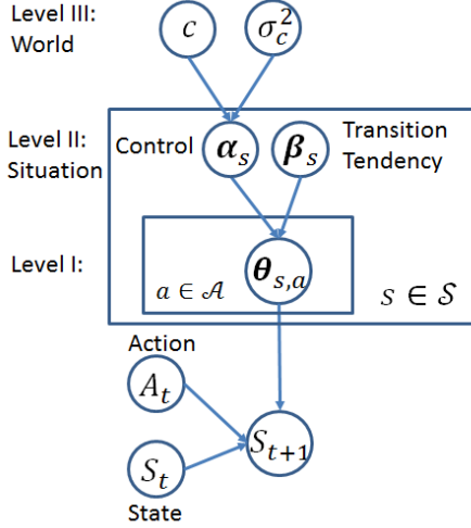
Figure 1: Hierarchical Bayesian model of state-transitions and controllability. \theta_{s,a} are the transition probabilities for taking action a in state s (level I). The second level, abstracts away from particular actions and represents the general outcome tendency \beta_s of situation s and its controllability \alpha_s . The third level abstracts away from any particular state and represents how controllable the world is in general ( c ) and how much states differ with respect to controllability ( \sigma_c^2 ).
