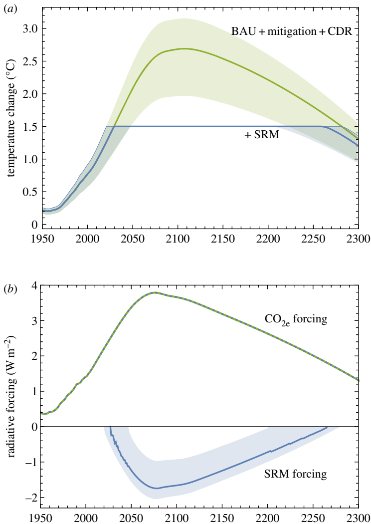
Figure 4. Uncertainty in climate sensitivity results in a range of temperature outcomes for a given \text{CO}_2 -concentration pathway; the multi-model median response and range across the 12 models considered here is shown for the case with long-term \text{CO}_2 removal both with and without solar geoengineering. (a) Solar geoengineering could be used to achieve a 1.5^\circ\text{C} target independent of climate sensitivity uncertainty. (b) The range of forcing from solar geoengineering across the 12 models and from \text{CO}_{2e} ; analysis uses % solar reduction and concentration, respectively, but these are plotted as approximate radiative forcing to enable comparison between them. \text{CO}_2 forcing is estimated as 5.35 times the log of the concentration change. Because of the short timescales associated with solar geoengineering, uncertainty in climate response can be compensated for with control over solar geoengineering forcing. (Online version in colour.)
