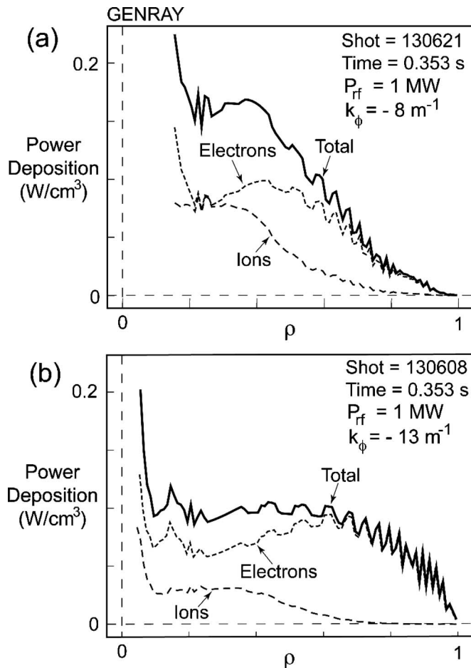
FIG. 11. Power deposition profiles calculated by GENRAY for I_p=1 MA, B_T(0)=0.55 T deuterium H-mode plasmas with 1 MW of (a) k_\phi=-8 \text{m}^{-1} (shot 130621) and (b) k_\phi=-13 \text{m}^{-1} heating (shot 130608).
