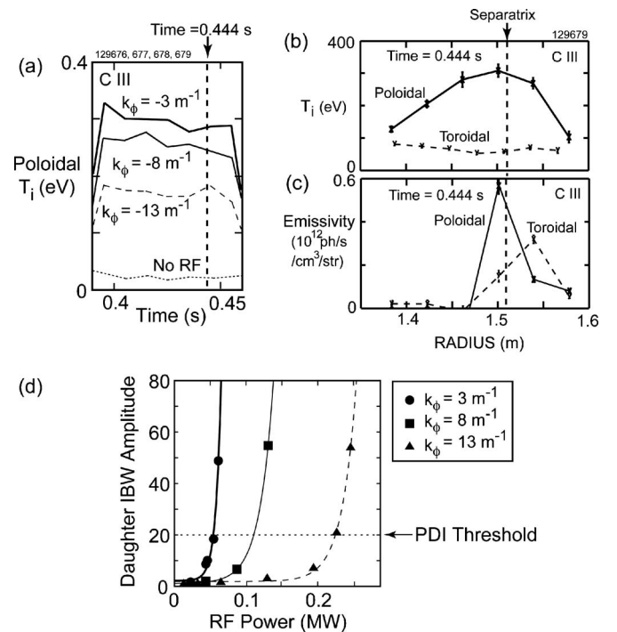
FIG. 8. Anisotropic C III ion heating measured near the plasma separatrix by passive ion spectroscopy. (a) Poloidal ion temperature at a major radius, R=1.500 m during 1.2–1.3 MW of k_\phi=-3 \text{ m}^{-1} (thick solid line, shot 129679), k_\phi=-8 \text{ m}^{-1} (thin solid line, shot 129678), k_\phi=-13 \text{ m}^{-1} (dashed solid line, shot 129676) rf heating of I_p=650 kA, B_T(0)=0.55 T deuterium discharges. Also included is a shot with no rf power (shot 129677, dotted line). For the case with k_\phi=-3 \text{ m}^{-1} heating at 0.444 s, radial profiles of (b) poloidal (solid line) and toroidal ion temperature (dashed line), and (c) poloidal (solid line) and toroidal (dashed line) C III emissivity. (d) Results from a one-dimensional full wave model of the PDI-generated IBW amplitude vs pump field and rf power.
