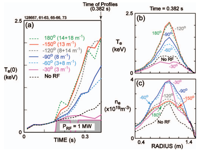
FIG. 2. (Color) (a) Time evolution of the T_e(0) , measured by MPTS, for a sequence of deuterium plasmas with I_p=600 kA, B_T(0)=0.55 T, 1 MW of rf power starting at 0.15 s, and no Li conditioning. \Delta\phi was adjusted from -30^\circ to 180^\circ in 30^\circ increments between shots. T_e(0) time evolution for a plasma without rf heating (black dashed line) is also plotted for comparison. Note the plasma with \Delta\phi = -30^\circ had an rf arc at 0.22 s. (b) T_e(R) and (c) n_e(R) measured by MPTS at 0.382 s during each discharge shown in Fig. 2(a).
