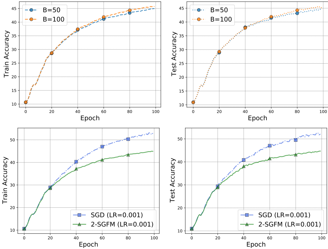
Figure 9.5: Additional experimental results on the CIFAR10 dataset [Krizhevsky and Hinton, 2009]. (Above) Performance of 2-SGFM with different choices of B . (Bottom) Performance of 2-SGFM and SGD.
