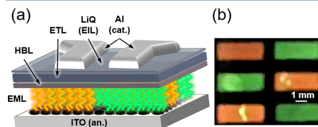
Figure 8. Multicolored OLED composed of poly(M6MA-co-IrppqMA) and poly(M6MA-co-IrppyMA) as the orange and green emitting regions, respectively. (a) Device architecture fabricated from the bottom up: ITO/EML/HBL/ETL/LiQ/Al. (b) Photograph showing electroluminescence of device under forward bias.
