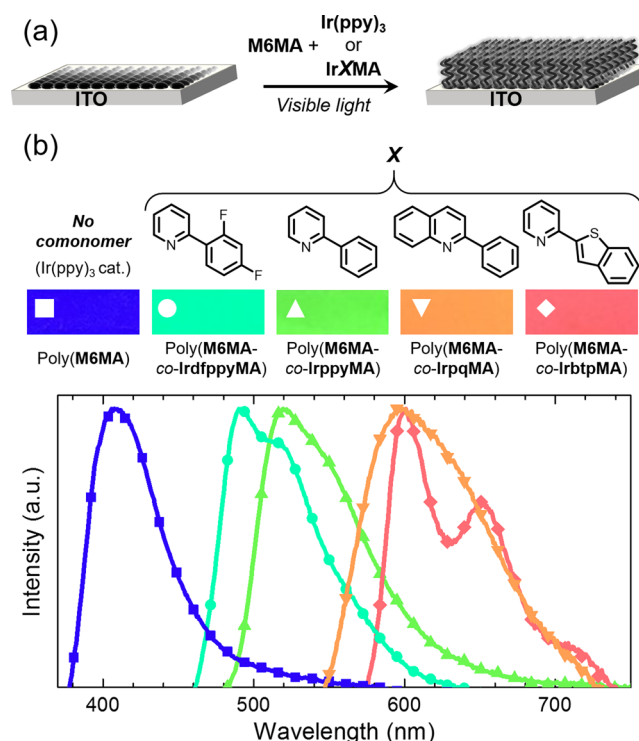
Figure 1. Polymer brushes grafted from ITO using \text{Ir}(\text{ppy})_3 (0.005 mol %) as the photocatalyst for poly( M6MA ) and 3 mol % IrXMA for copolymers. (a) Schematic representation of grafting from procedure; initiator functionalized ITO to polymer brushes. (b) Chemical structures for C N ligands (X) of IrXMA and corresponding photoluminescence profiles. Rectangles are images of the polymer brushes on ITO under 365 nm excitation (Figure S14 for full images).
