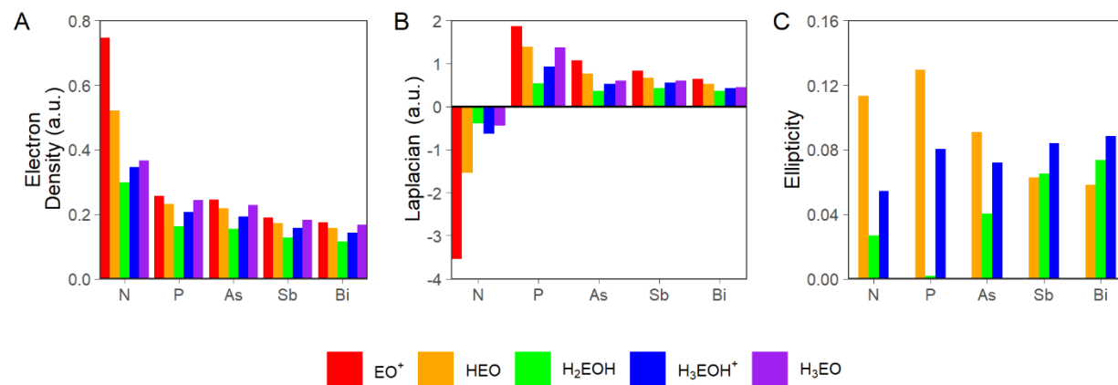
Figure 2. Values of (A) \rho_b , (B) \nabla^2\rho_b , and (C) \varepsilon_b for all 15 species grouped by pnictogen and colored by compound type. For (C), note that all \text{EO}^+ and \text{H}_3\text{EO} compounds have \varepsilon_b = 0 . Note that \rho_b ,
