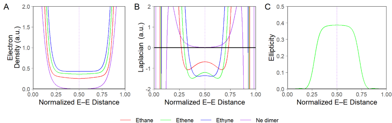
Figure 1. Plots of (A) \rho , (B) \nabla^2\rho , and (C) \epsilon as a function of the normalized C–C (for ethane, ethene, and ethyne) or Ne–Ne (for Ne dimer) bond length for a series of reference compounds. For (C), note that ethane, ethyne, and \text{Ne}_2 have \epsilon = 0 along the length of the bond. Orbital-optimized electron densities were obtained from single-point CCSD/ANO-RCC-QZP calculations at experimental geometries extracted from the NIST CCCDB. 43 See Figure S2 for CVD balanced image.
