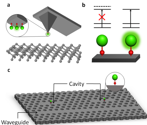
Figure 6. Applications of surface bound OCCs. (a) An AFM/STM tip can be functionalized with OCC centers, enabling precision quantum-enhanced readout of local magnetic and electric fields through fluorescence. (b) Two OCCs in spatial proximity can provide the two qubit basis for a CNOT gate achieved through dipole blockade. (c) OCCs can be placed in a photonic waveguide, entangling two OCCs via photonic bus.
