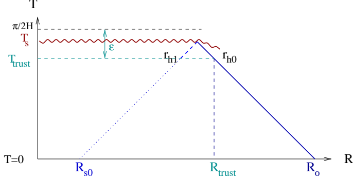
Fig. 4: “Causal” diagram in FRW coordinates (figure not to scale) for obtaining estimates of the horizon size.
