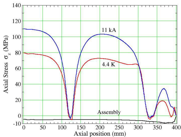
Fig. 9. Calculated axial stress showing a dips in the island gaps.
