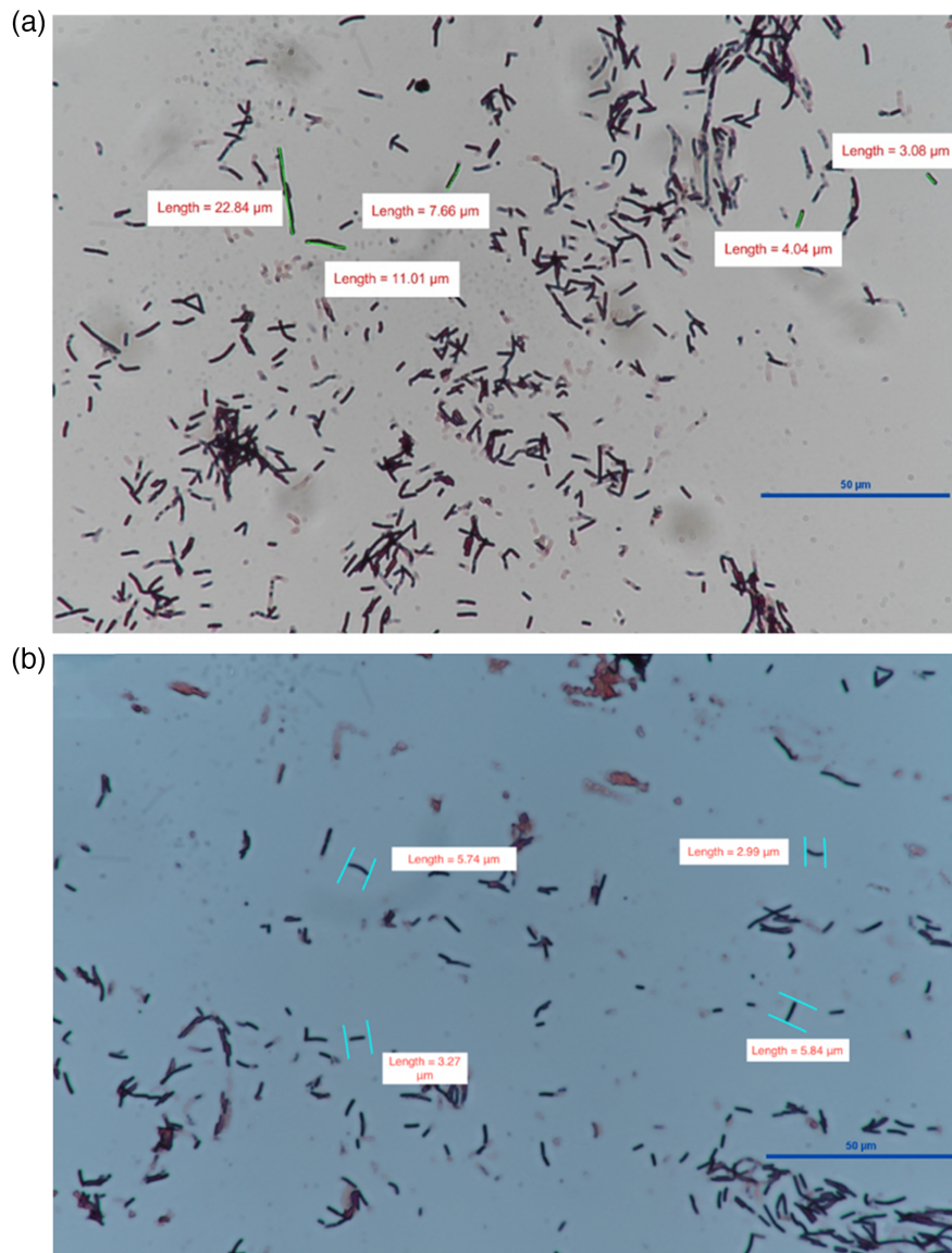
Fig. 2 Bacterial gram stains: (a) image of a gram stain of colonies with no heating and (b) image of a gram stain of colonies after heating. Average bacterial length before and after heating were 7.42 \pm 0.6 microns and 4.8 \pm 0.8 microns, respectively ( p = 0.038 ). The scale bar in both images is 50 \mu\text{m} .
