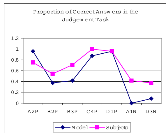
Figure 3: Proportions of correct answers in the judgment task. A2P through D1P are the five "on" relations of the system, A1N and D3N the two "off" relations. (A2P: Switch A – Lamp 2 - positive)
