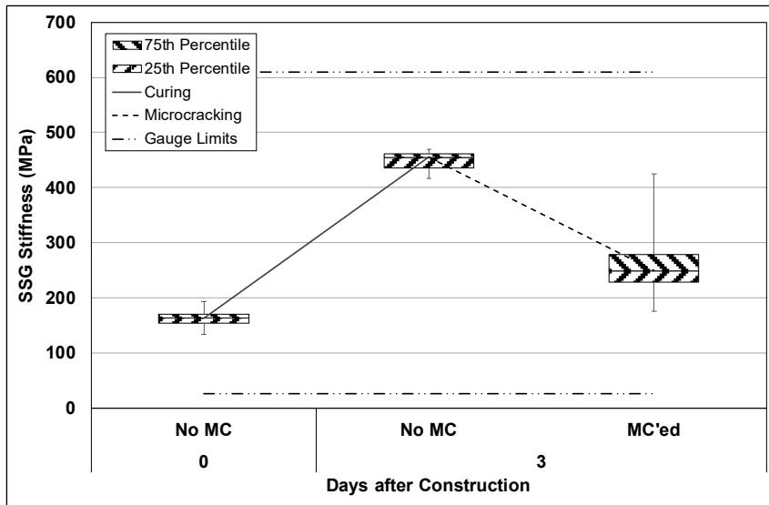
Figure B.204: Cell S27: SSG measured stiffness.
