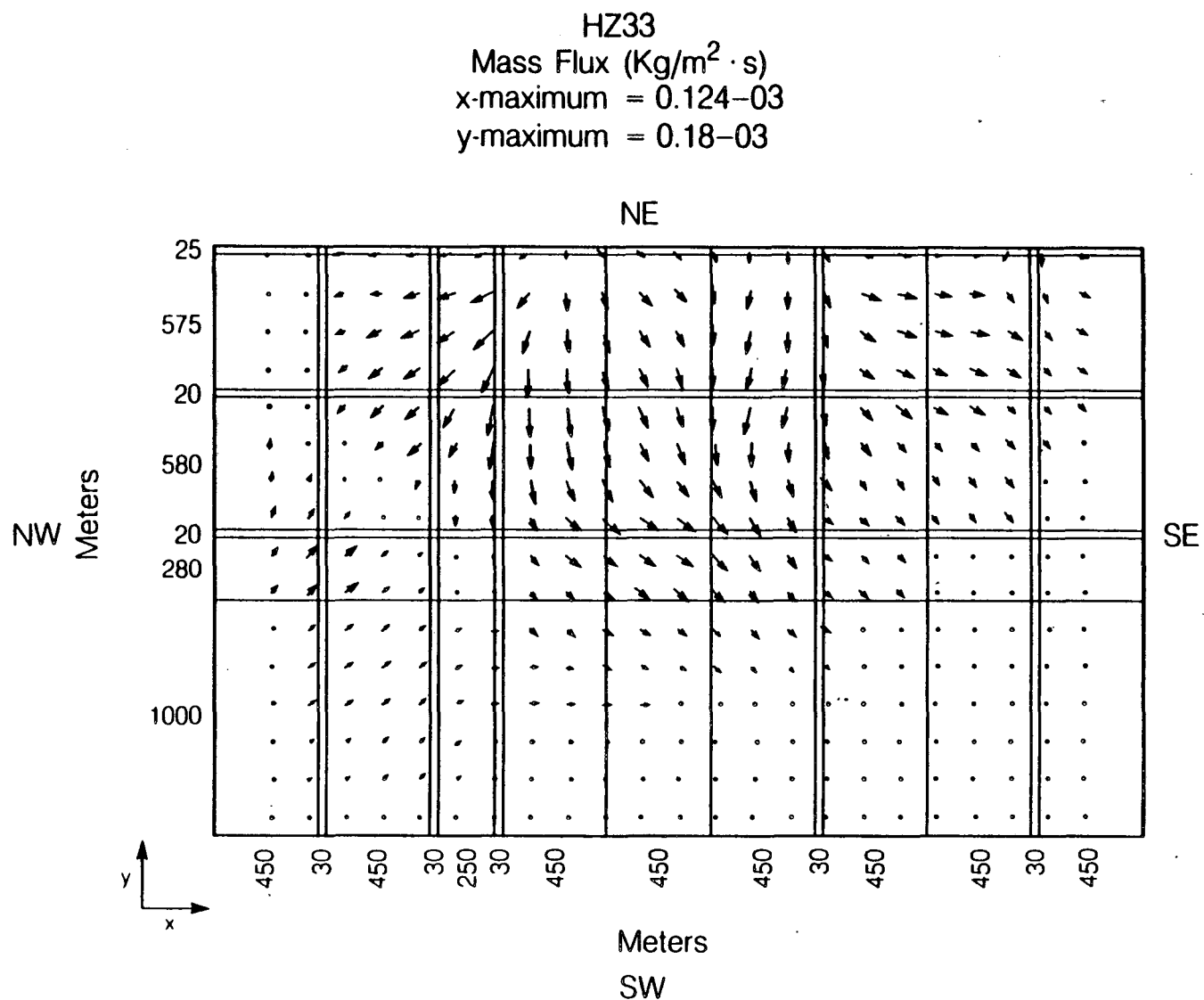
Figure 56. Mass flux plots for horizontal section, HZ33. Mass flux is in ( \text{kg}/\text{m}^2 \cdot \text{s} ).
