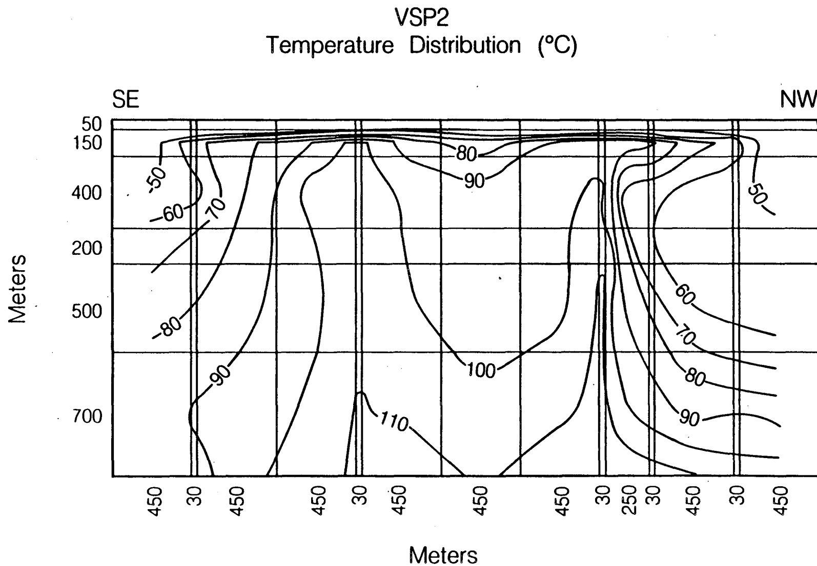
Figure 43. Temperature distribution for vertical sections VSP2, parallel to the main normal fault. Temperatures are in (°C).
