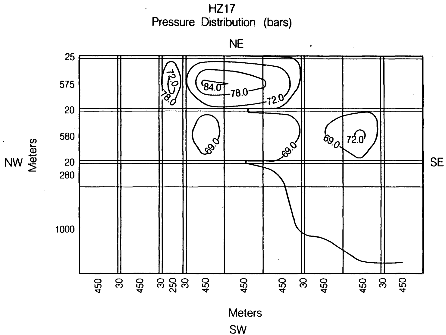
Figure 41b. Pressure distribution for horizontal section, HZ17. Pressures are in (Bars).
