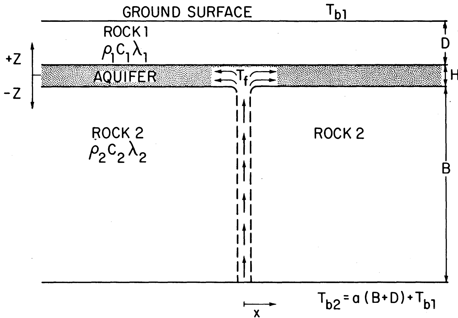
Figure 19. Fault-charged model showing important parameters (taken from Bodvarsson et al., 1982).
