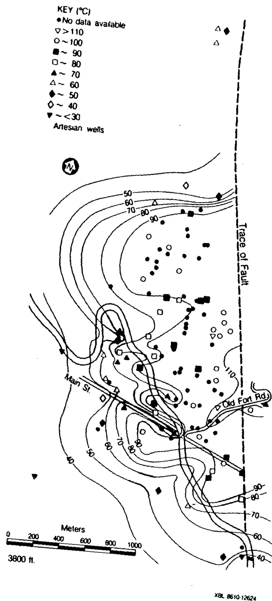
Figure 16a. Temperature contour plots drawn at elevations 3600 ft, 3700 ft and 3800 ft a.s.l.
