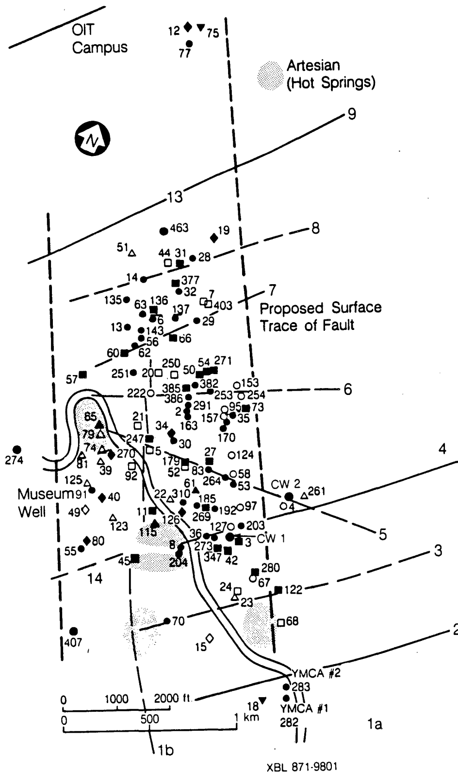
Figure 15. Fault locations inferred from the cross-sectional temperature profiles and temperature contour plots. Solid lines indicate a higher degree of certainty.
