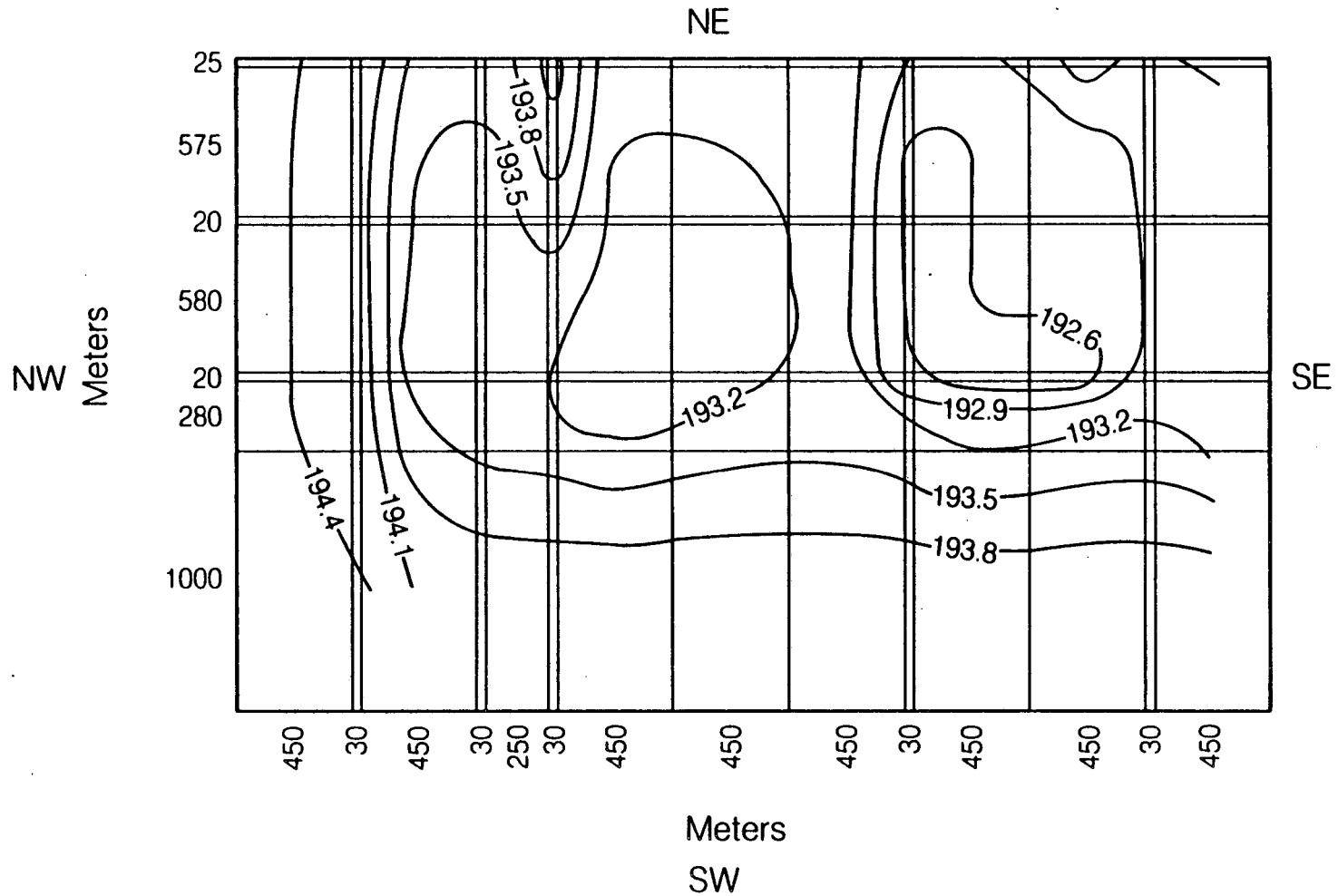
Figure 34a. Bottom Boundary pressure distribution (Bars).
