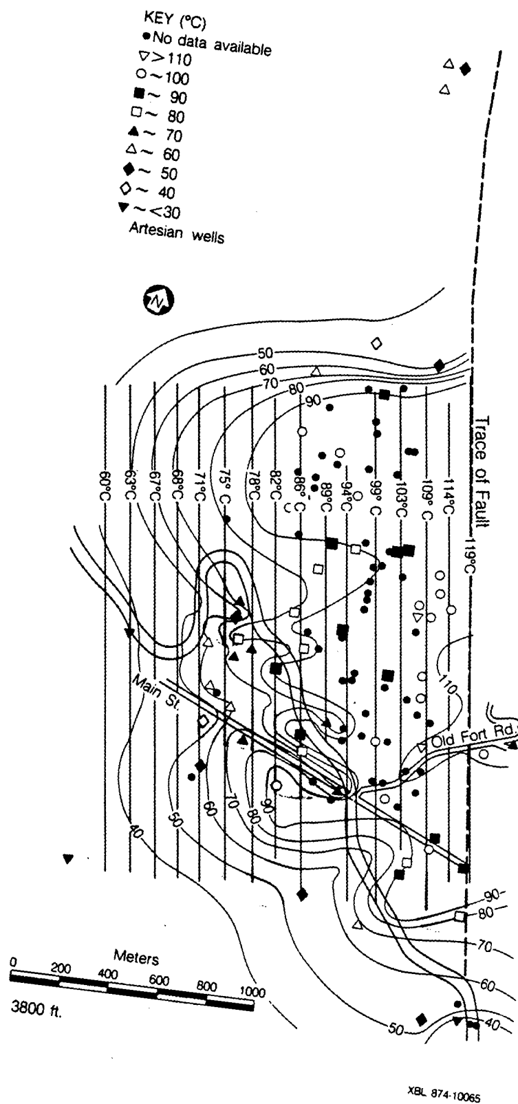
Figure 20a. Calculated and actual field data comparison for the fault-charged model.
