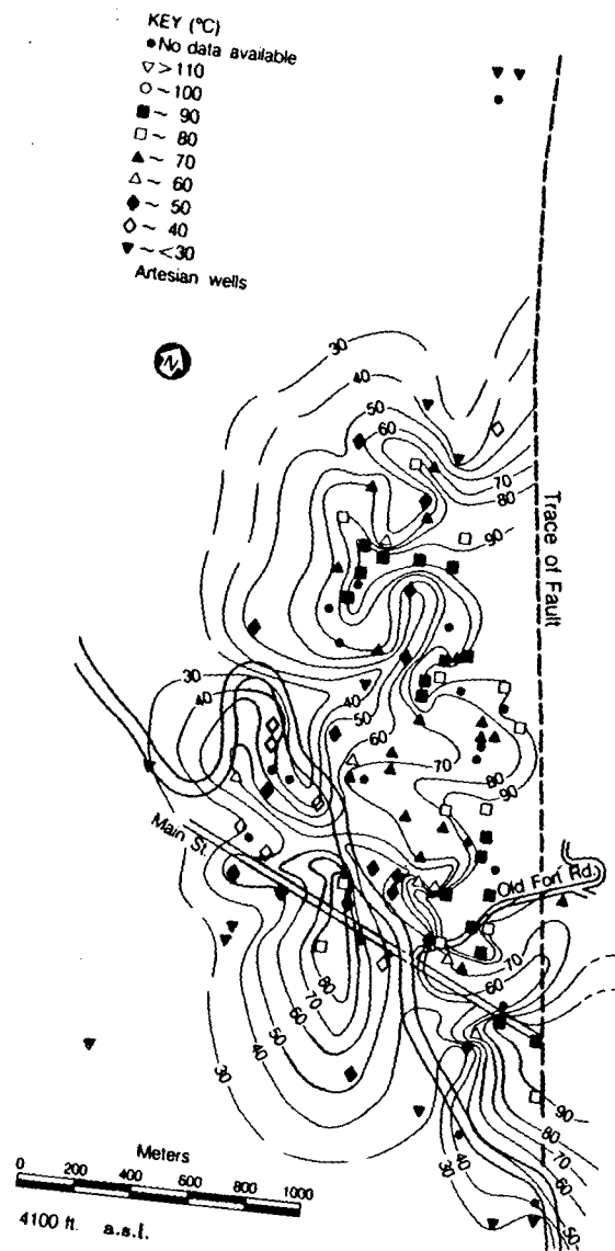
Figure 16b. Temperature contour plots drawn at elevations 3900 ft, 4000 ft and 4100 ft a.s.l.
