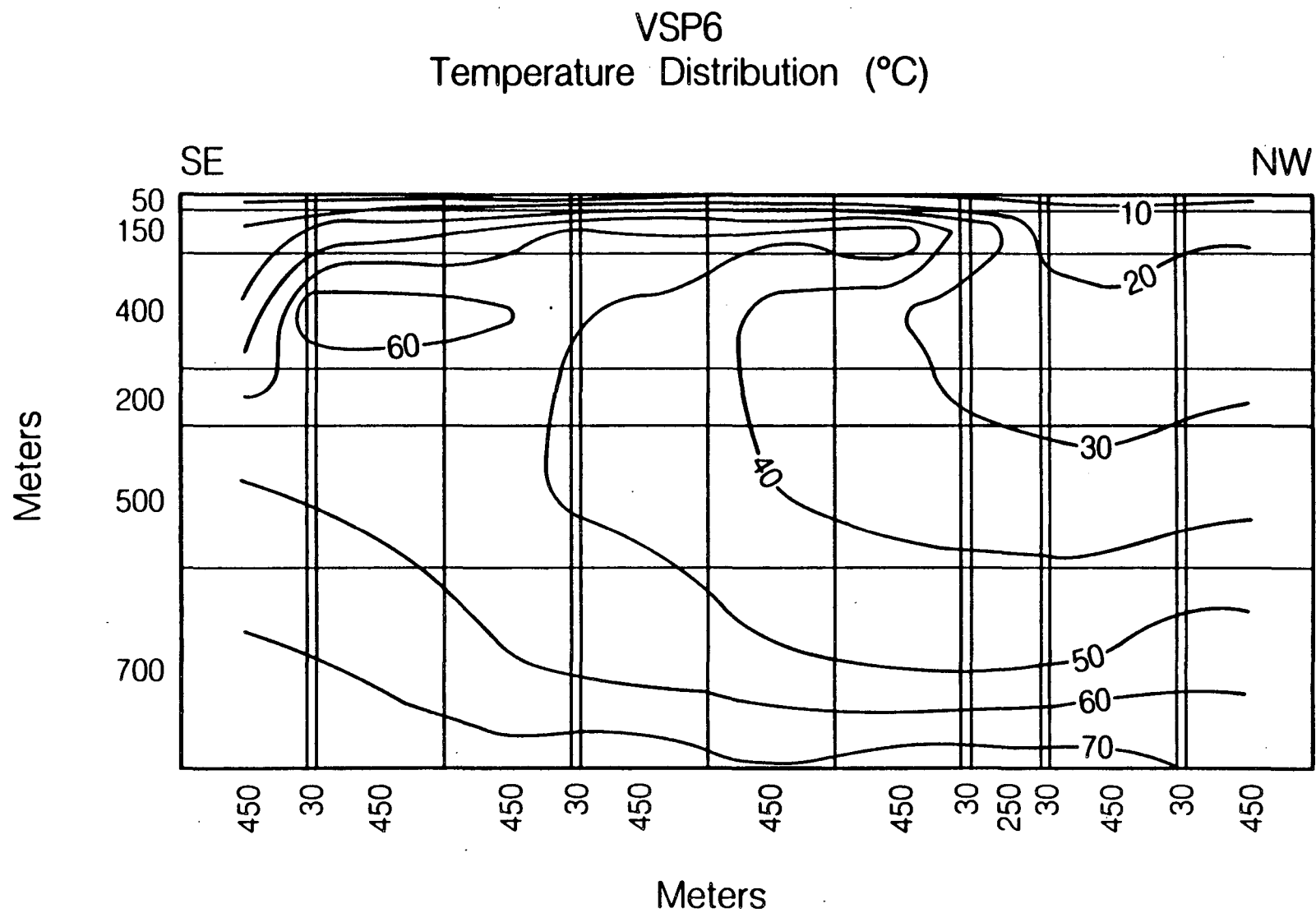
Figure 45. Temperature distribution for vertical sections VSP6, parallel to the main normal fault. Temperatures are in (°C).
