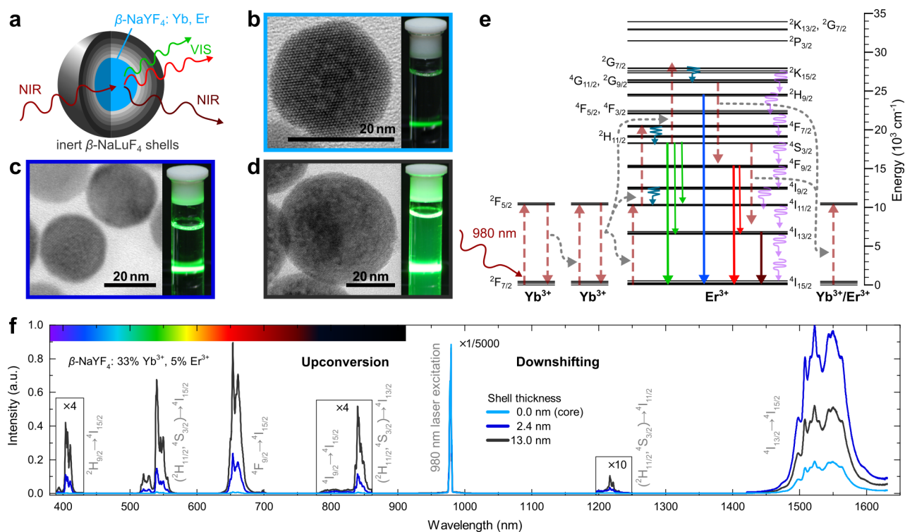
Figure 1. Efficient visible upconversion and near-infrared downshifting in \beta -NaYF 4 : Yb 3+ , Er 3+ @NaLuF 4 core-shell nanocrystals. (a) Design of core-shell particles using the same \beta -NaYF 4 : Yb 3+ , Er 3+ core but different \beta -NaLuF 4 shell thicknesses. (b–d) TEM images of the \beta -NaYF 4 : Yb 3+ , Er 3+ core as well as core-shell nanocrystals with a 2.4 and 13.0 nm thick \beta -NaLuF 4 shell, respectively. All scale bars are 20 nm. The photographs show the bright visible upconversion under 980 nm laser excitation with 63 W/cm 2 . (e) Schematic representation of the upconversion and downshifting process under 980 nm excitation. The incident photons are predominantly absorbed by Yb 3+ and the energy is transferred to Er 3+ . However, the excitation energy migrates through the entire core nanocrystal by efficient hopping from one Yb 3+ ion to another neighboring Yb 3+ . (f) Emission spectrum of bright upconversion at shorter wavelengths and simultaneously strong NIR downshifting luminescence from Er 3+ 4 I 13/2 energy level for the three samples shown in panels b–d.
