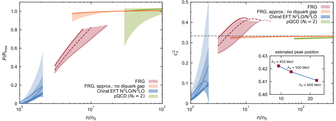
FIG. 1. Left panel: Pressure P of symmetric nuclear matter normalized by the pressure of the free quark gas P_{\text{free}} as a function of the baryon density n/n_0 in units of the nuclear saturation density as obtained from chiral EFT, FRG, including results from an approximation without taking into account a diquark gap (FRG, approx.: no diquark gap), and pQCD, see main text for details. Right panel: Speed of sound squared as a function of the baryon density in units of the nuclear saturation density as derived from the pressure shown in the left panel. The inset shows the estimated peak position and height for different transition scales \Lambda_0 as obtained by increasing the chemical potential \mu beyond \Lambda_0 .
