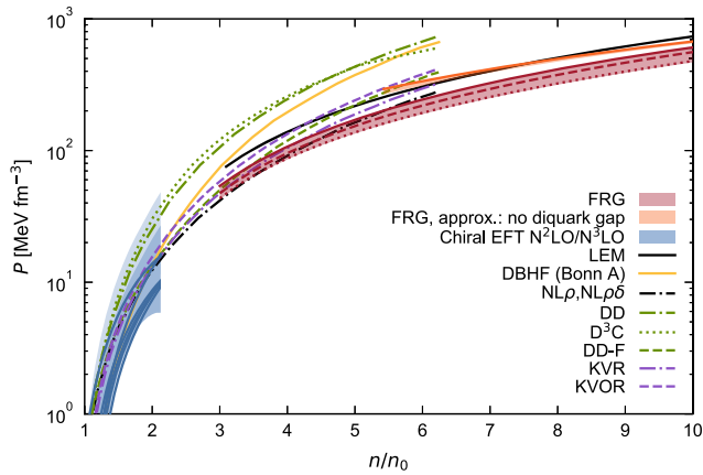
FIG. 2. Pressure of symmetric nuclear matter as obtained from chiral EFT, FRG, and pQCD, as in Fig. 1, in comparison with different models (see main text and also Ref. [35]).
