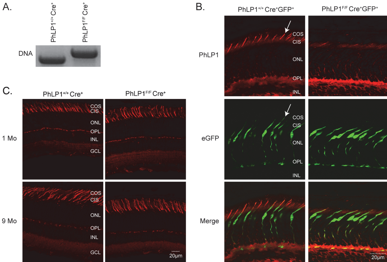
Fig 1. Characterization of the cone photoreceptor-specific PhLP1 knockout mouse. A) PCR genotyping results using the PhLP F primers. The PhLP1 F gene generated a 704 bp product, while the wild-type gene generated a 600 bp product. B) Immunolocalization of PhLP1 in retinal cross-sections from PhLP1 +/+ Cre + GFP + and PhLP1 F/F Cre + GFP + mice expressing EGFP in cones. Immuno-labeling with a PhLP1 primary antibody and AF555-conjugated secondary antibody is shown in red and the EGFP fluorescence is shown in green. These images were merged to show cone expression of PhLP1. C) TRITC-PNA (red) labeling of cones in retinal cross-sections from 1-month and 9-month-old PhLP1 +/+ Cre + and PhLP1 F/F Cre + mice.
