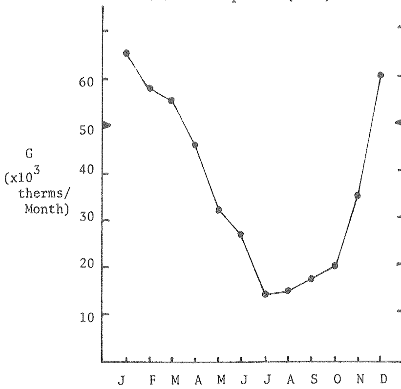
a. Gas Consumption (1976)
