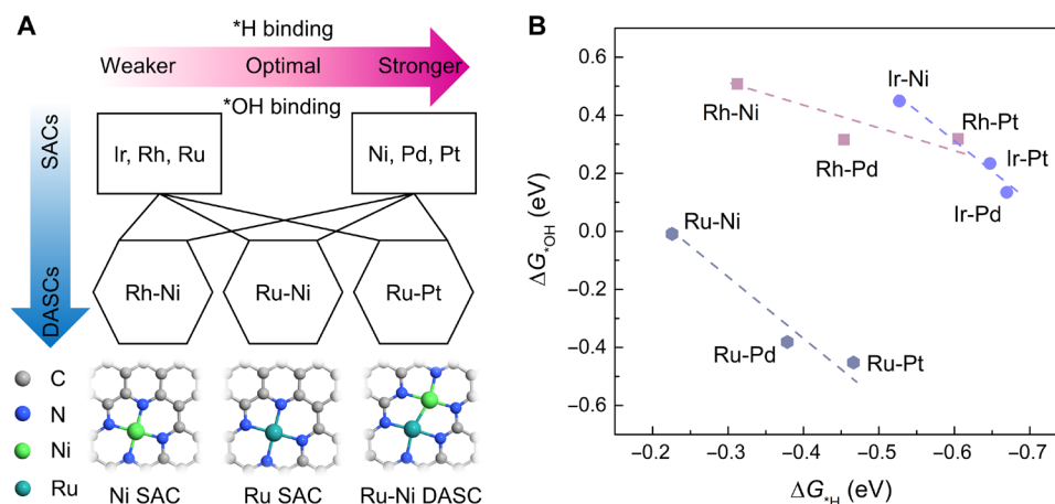
Fig. 1. Tuning the energetics of HOR reaction intermediates by DASCs. (A) Tuning the binding energy of *H ( \Delta G_{\text{H}} ) and *OH ( \Delta G_{\text{OH}} ) via a combination of various SACs. We categorized the SACs into two different groups: strong binding—Ir, Rh, and Ru; weak binding—Ni, Pd, and Pt. The optimized structures of Ni SAC, Ru SAC, and Ru-Ni DASC are illustrated (cyan, Ru; green, Ni; blue, N; and gray, C). (B) \Delta G_{\text{H}} and \Delta G_{\text{OH}} of different DASCs determined by Bayesian error estimation functional with van der Waals calculations with the optimum values obtained for Ru-Ni DASC on the basis of the Sabatier principle.
