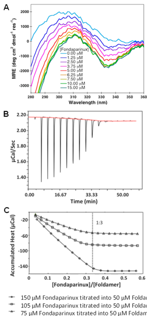
Figure 6. Near UV CD and ITC characterizations of SalAA compound 1 binding to fondaparinux. (A) Near UV CD spectra of the fondaparinux titration of compound 1 , (Lys-Sal) 4 -CONH 2 , where increasing concentrations of fondaparinux were titrated into 25 \mu M compound 1 . (B) Concentration-dependent ITC of fondaparinux titrated into compound 1 , (Lys-Sal) 4 -CONH 2 . Shown are the raw data of 150 \mu M fondaparinux (stock solution) titrated into 50 \mu M compound 1 . (C) Accumulated integrated heat changes as a function of fondaparinux:foldamer molar ratio for three experiments at the listed concentrations.
