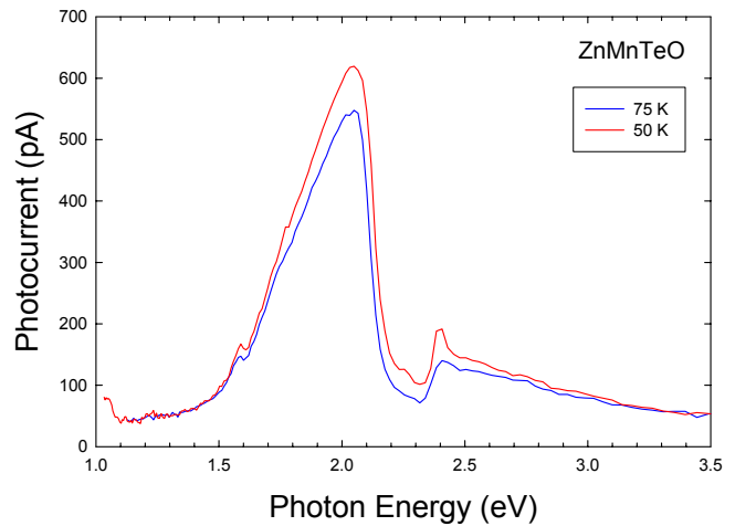
Figure 2. Photocurrent from ZnMnTeO synthesized by PLM at a fluence of 0.3 \text{ J/cm}^2 .
