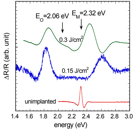
Figure 1. Photomodulated reflectance (PR) spectra obtained from \text{Zn}_{0.88}\text{Mn}_{0.12}\text{Te} samples as-grown and implanted with 3.3% \text{O}^+ followed by PLM with energy fluence of 0.15 and 0.3 \text{ J/cm}^2 .
