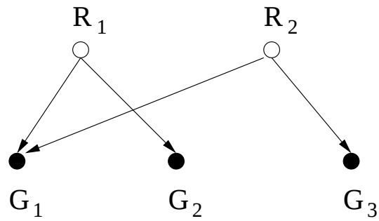
Figure 1: A network for transcription regulations. Parent nodes, indicated as empty circles, represent regulatory proteins, or transcription factors. Descendants, filled circle, targeted genes.
