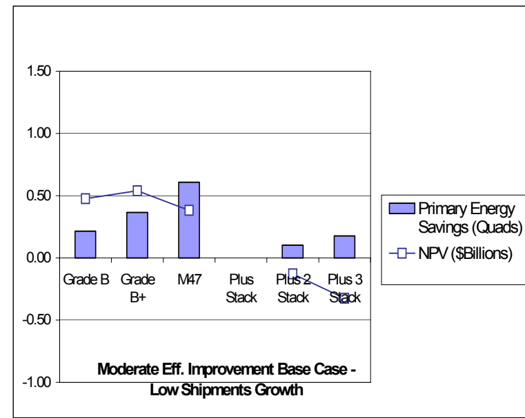
Figure ES-1 Cumulative Primary Energy Savings and Net Present Value of Energy Efficiency Improvement for Capacitor Start Motors, Based on LBNL Engineering Calculations
