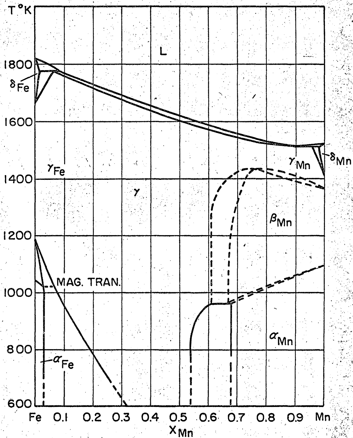
FIG. 4 IRON-MANGANESE SYSTEM. (22)
