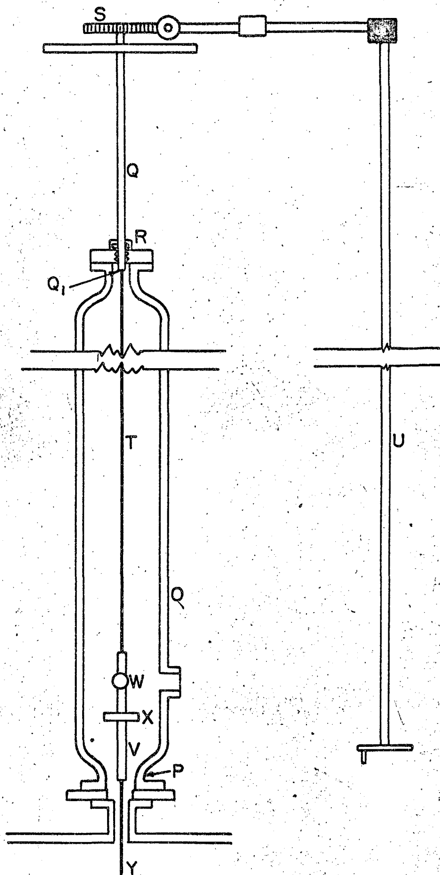
FIG. 2 SUSPENSION SYSTEM.
