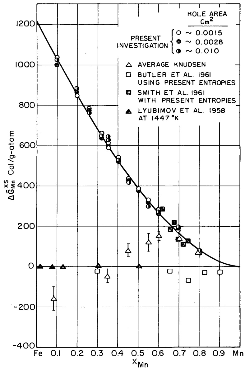
FIG. 12 \Delta \bar{G}_{\text{Mn}}^{\text{xs}} FOR SOLID IRON-MANGANESE ALLOYS WITH RESPECT TO \gamma_{\text{Mn}} AT 1450 °K.
