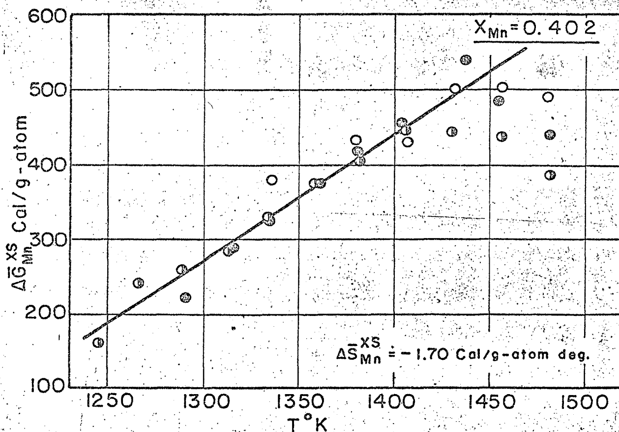
FIG. 7 EXPERIMENTAL VALUES OF \Delta \bar{G}_{Mn}^{XS} FOR SOLID IRON-MANGANESE ALLOYS WITH RESPECT TO \gamma_{Mn} .
