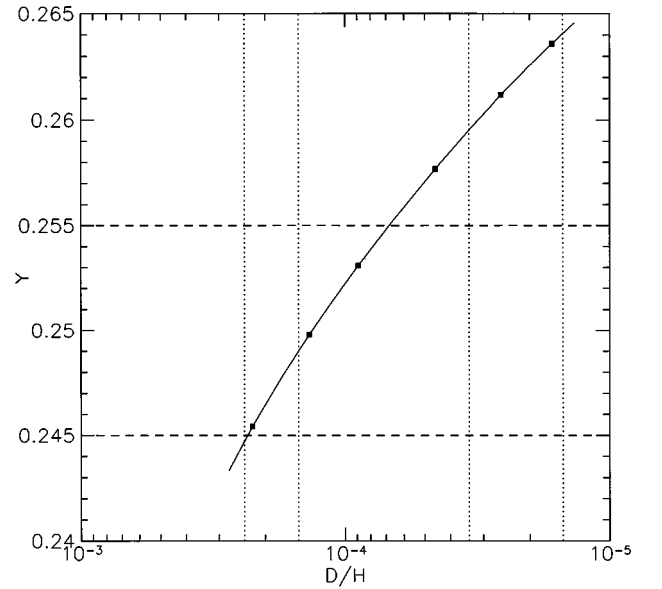
FIG. 1. BBN yields for a typical \nu_\mu - \nu_s atmospheric neutrino solution ( \delta m^2 = 1.0 \times 10^{-2} eV 2 , \sin^2 2\theta = 0.6 ). The solid curve is the 4 He mass fraction Y vs D/H. The squares indicate, from lower left to upper right, 10^{10} \eta = 1.7, 2.3, 3.0, 4.6, 6.6, 8.6 . The dotted lines indicate the ranges of “high” and “low” D/H inferred from QAS studies. The dashed lines indicate two possible upper limits on Y : the currently popular Y = 0.245 , and the more conservative Y = 0.255 .
