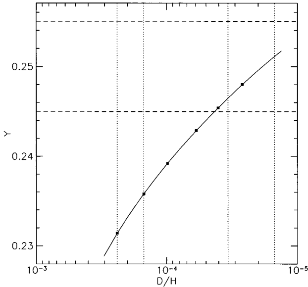
FIG. 2. BBN yields for a typical \nu_e - \nu_s small-angle MSW solution to the solar neutrino problem ( \delta m^2 = 4.0 \times 10^{-6} eV 2 , \sin^2 2\theta = 8.0 \times 10^{-3} ). The solid curve is the 4 He mass fraction Y vs D/H . The squares indicate, from lower left to upper right, 10^{10}\eta = 1.5, 2.0, 2.6, 3.6, 4.6, 5.6 . The dotted lines indicate the ranges of ‘‘high’’ and ‘‘low’’ D/H inferred from QAS studies. The dashed lines indicate two possible upper limits on Y : the currently popular Y = 0.245 , and the more conservative Y = 0.255 .
