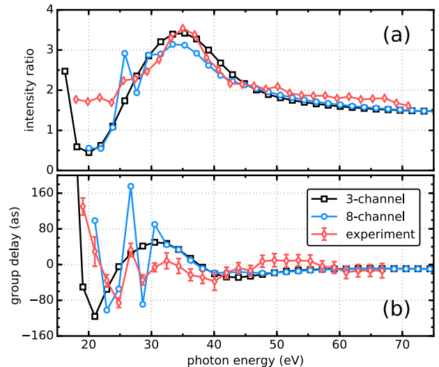
FIG. 4. (Color online) Complex dipole of N 2 along the internuclear axis. Direct comparison between experiment and 3- and 8-channel model of the dipole normalized intensity (a) and group delay (b) for the ensemble of N 2 aligned at 0°.
