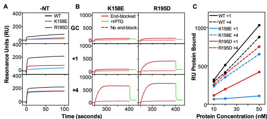
FIGURE 7. The Msh3 K158E and R195D mutations differentially affect binding to small versus large insertion-containing mispairs. A, the binding of wild-type Msh2-Msh3 (black) and the Msh2-Msh3-K158E (blue) and Msh2-Msh3-R195D (red) mutant complexes (50 nM) to homoduplex DNA and substrates containing a +1 or +4 insertion/deletion mispairs was monitored using SPR as described under “Experimental Procedures” in the absence of added nucleotide (–NT). B, sliding clamp formation by the Msh2-Msh3-K158E and Msh2-Msh3-R195D mutant complexes (50 nM) on the indicated substrates was monitored in the presence of ATP by SPR. The sensorgrams show the binding to substrates with free ends (dashed red lines) or ends blocked by bound LacI (solid red) followed by release of the end block (green) by the addition of IPTG. C, comparison of the binding of wild-type Msh2-Msh3 (black) and the K158E (blue) and R195D (red) mutant complexes to the +1 (solid lines) and +4 (dashed lines) end blocked substrates at different protein concentrations. The RUs observed immediately before IPTG addition are plotted.
