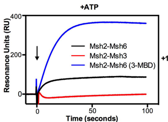
FIGURE 6. The low steady-state binding in the presence of ATP is not dependent on the Msh2-Msh3 mispair-binding domain. The binding of Msh2-Msh3 (red), Msh2-Msh6 (black), and the chimeric protein Msh2-Msh6(3-MBD) (blue) to the +1 insertion/deletion mispair and the homoduplex substrate was monitored using SPR analysis as described under "Experimental Procedures" in the presence of ATP (+ATP). The sensorgram shows the binding to +1 after subtraction of the RUs observed on the homoduplex substrate. The x axis indicates the time of association in seconds, the y axis indicates the extent of binding in RUs, and the black arrow indicates the time at which the injection of protein was initiated.
