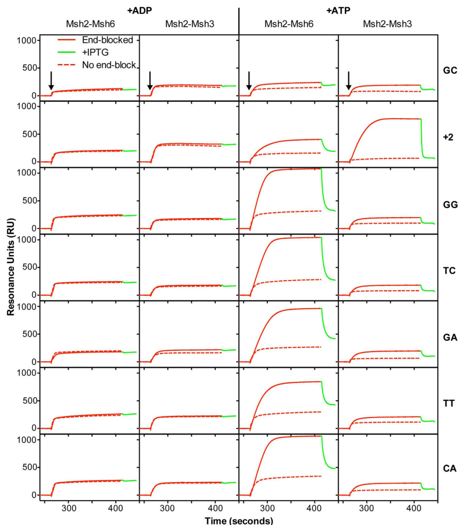
FIGURE 5. Msh2-Msh3 forms ATP-dependent sliding clamps on substrates containing insertion/deletion mispairs and specific base-base mispairs. See the legend to Fig. 4 for experimental details and a key for abbreviations used.
