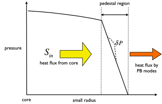
FIG. 1 (color online). Setup of the analysis.
