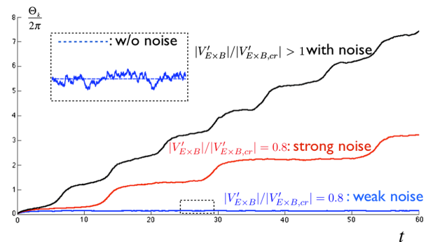
FIG. 4 (color online). Noise effects on cross phase dynamics.
