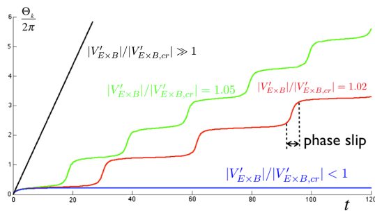
FIG. 2 (color online). Phase locked (blue plot) vs phase slip (green and red plots).
