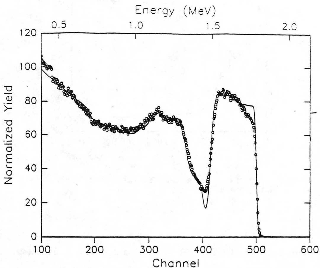
Figure 37. RBS data (circles) of a KTN/LSC/LAO heterostructure grown at 675 °C. The data simulation (line) indicates that the KTN film is \sim 0.18 \mu\text{m} thick and has composition \text{K}_{.83}\text{Ta}_{.88}\text{Nb}_{.12}\text{O}_x .
