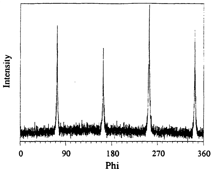
Figure 28. Phi-scan of a [100] perovskite KTN film grown on (100) p LAO at 600°C and 400 mTorr showing four-fold symmetry of the {111}.
