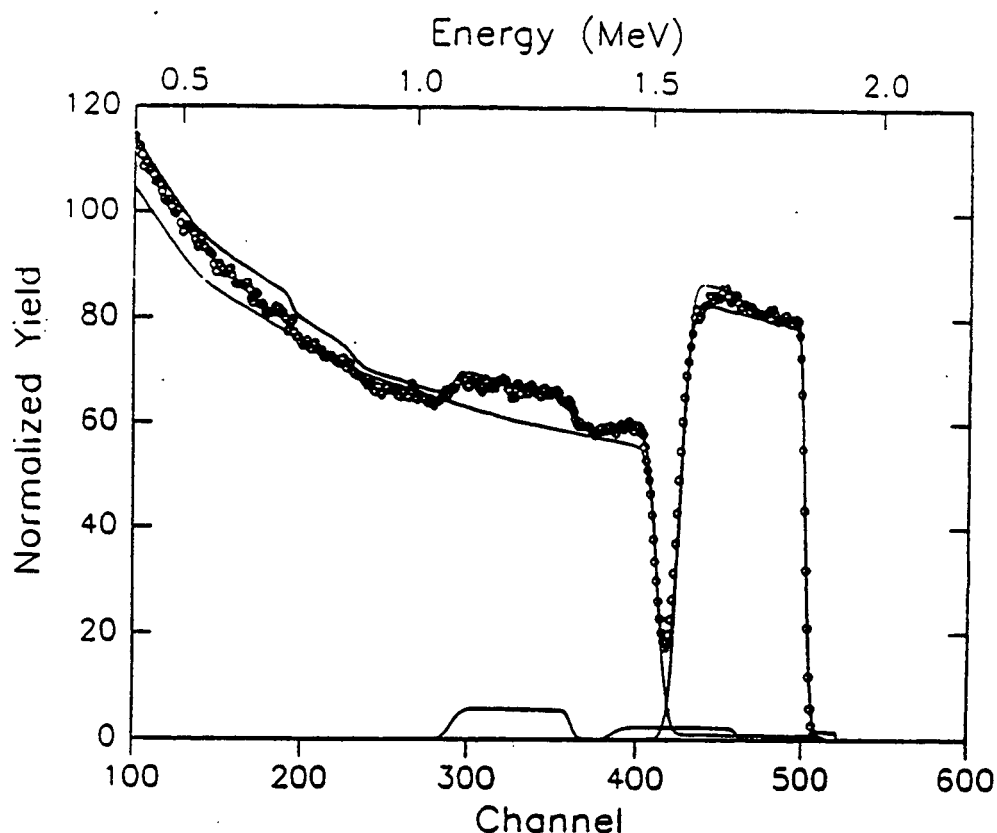
Figure 29. RBS raw data (circles) and fit (lines) for a KTN film grown on (100) p LAO at 700 °C and 400 mTorr. The fit resulted in a thickness of 0.28 \mu\text{m} and composition \text{K}_{0.9}\text{Ta}_{0.92}\text{Nb}_{0.08}\text{O}_x .
