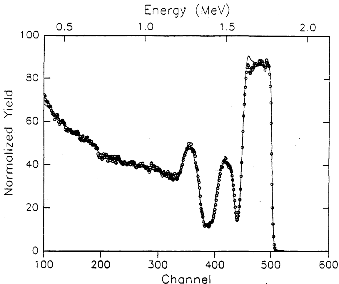
Figure 47. RBS measurement (circles) of a KTN/YBCO/STO heterostructure. The simulation (line) is for a KTN film thickness of 0.2 \mu\text{m} and composition of \text{K}_{0.78}\text{Ta}_{0.88}\text{Nb}_{0.12}\text{O}_3 .
