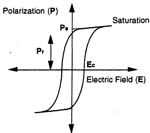
Figure 5. Polarization vs. electric field of a ferroelectric phase.
