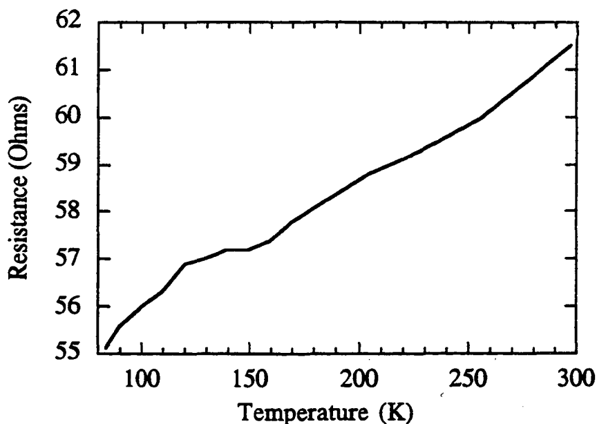
Figure 48. Resistance vs. temperature of YBCO bottom contact to a KTN/YBCO/LAO heterostructure grown at 675/760^\circ\text{C} . The YBCO is metallic.
