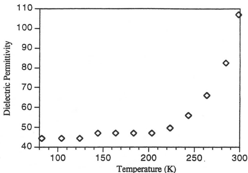
Figure 45. Dielectric permittivity vs. temperature for measured at 100 Hz and 301 \mu V A.C. signal of a KTN/LSC device grown on Pt/Ti/SiN/Si at 600 °C.
