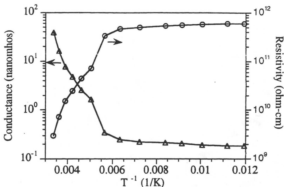
Figure 38. Conductance vs. temperature of a capacitive device from a KTN/LSC/LAO grown at 675 °C.
