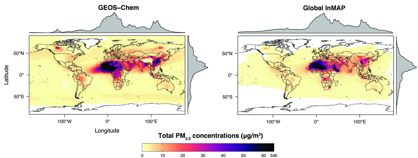
Fig 1. Annual-average ground-level total \text{PM}_{2.5} concentrations from the Global InMAP and GEOS-Chem simulations for year 2016.
