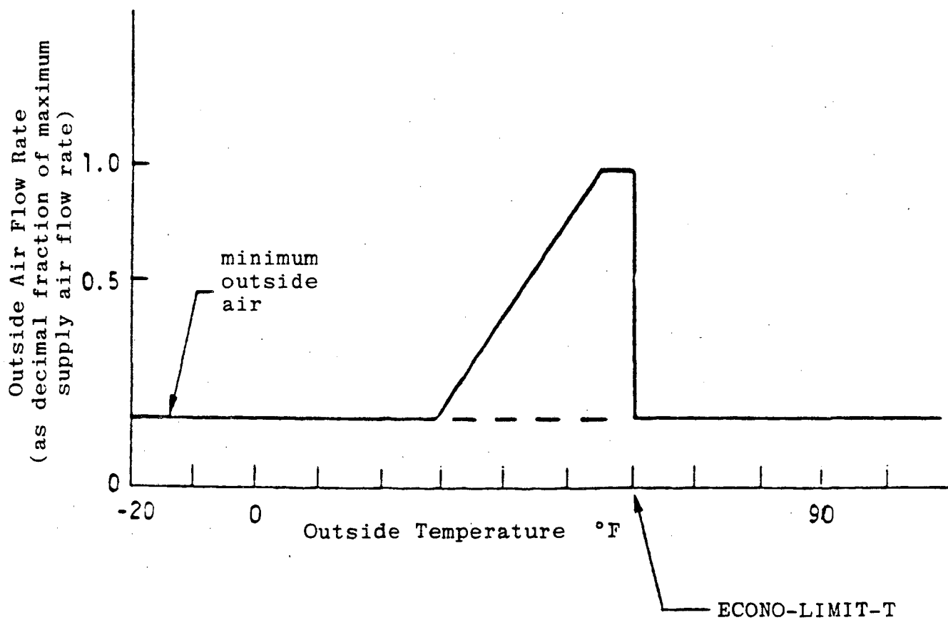
Figure 3.29: Typical curve of air flow vs outside air temperature for systems with temperature type economizer (illustrating use of keyword ECONO-LIMIT-T)
