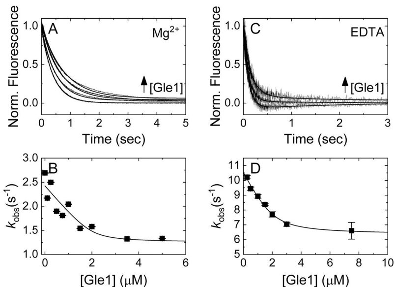
Figure 5. Gle1 slows mantADP( \pm Mg 2+ ) dissociation from Dbp5
