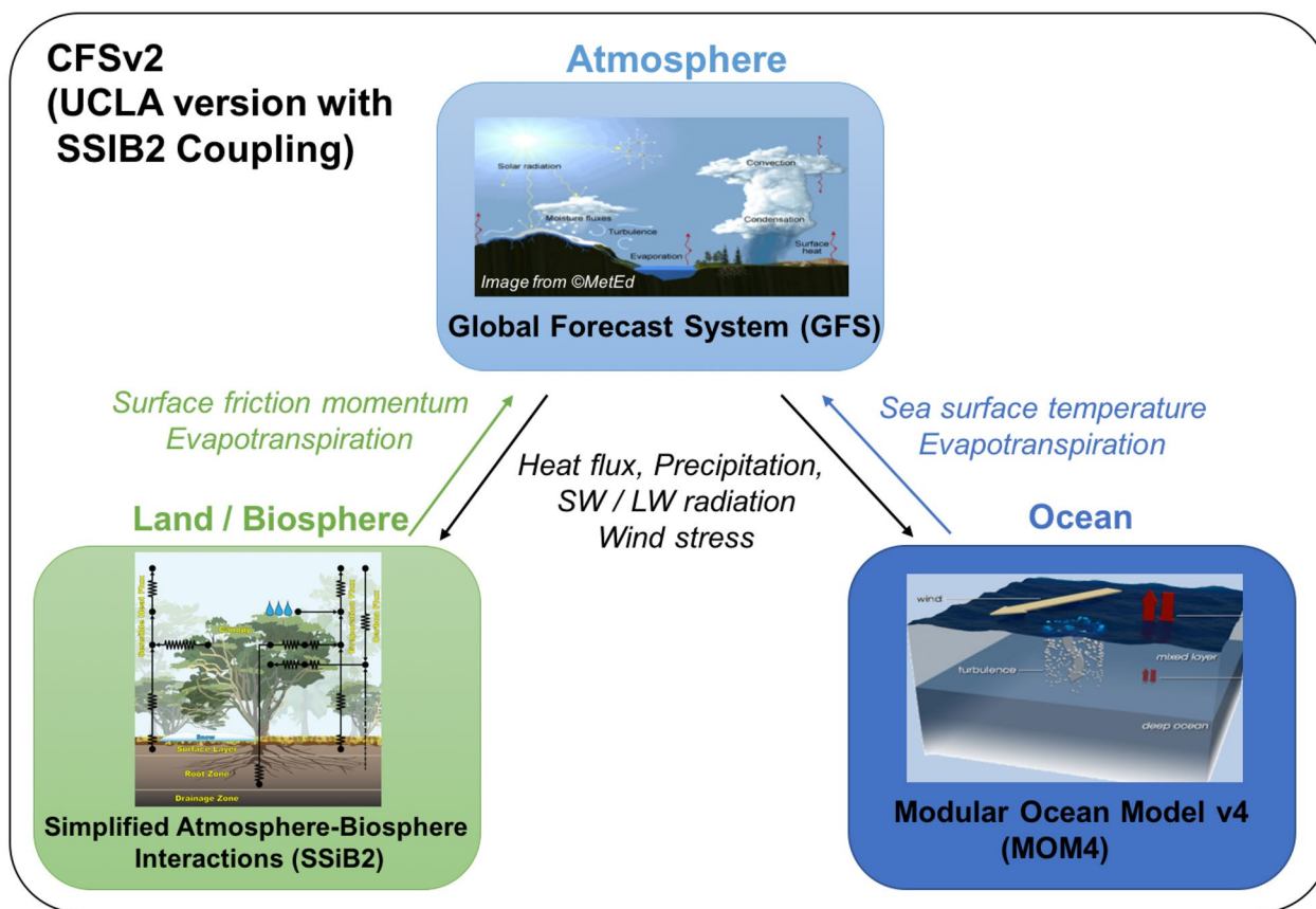
Fig. 1 Schematic diagram for the coupled numerical modeling system, CFSv2. The GFS, SSiB2, and MOM4 are respectively used for atmospheric, land-surface, and ocean modeling components. The arrows indicate ongoing exchange of variables between individual
