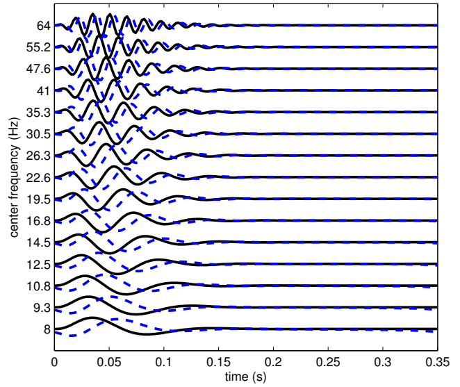
Fig. 2. Frame waveforms \mathbf{x} , black solid lines are real components \mathbf{m} and dashed blue lines are imaginary components derived from the Hilbert transform h(\mathbf{m}) . The length of the waveforms is 180.
