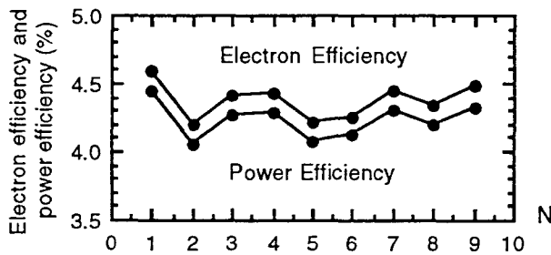
Figure 6. Electron efficiency \eta_e and power efficiency \eta_p versus cavity number N.
