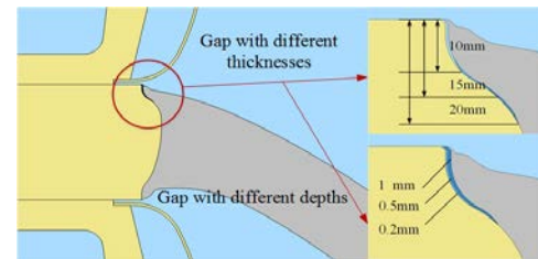
Figure 12. The air-gaps with different size at the interface
