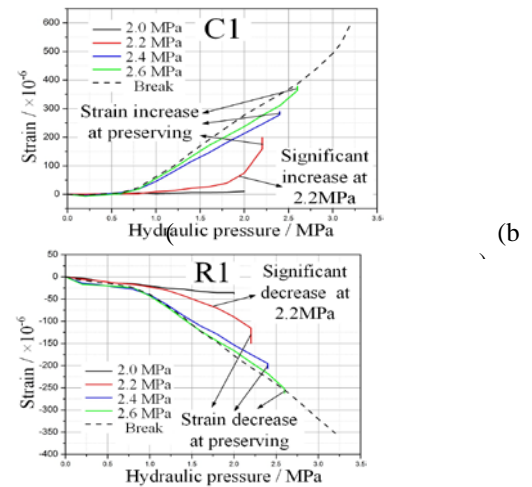
Figure 4. Strain of (a) C1 and (b) R1 sensors when abnormality occurs.
